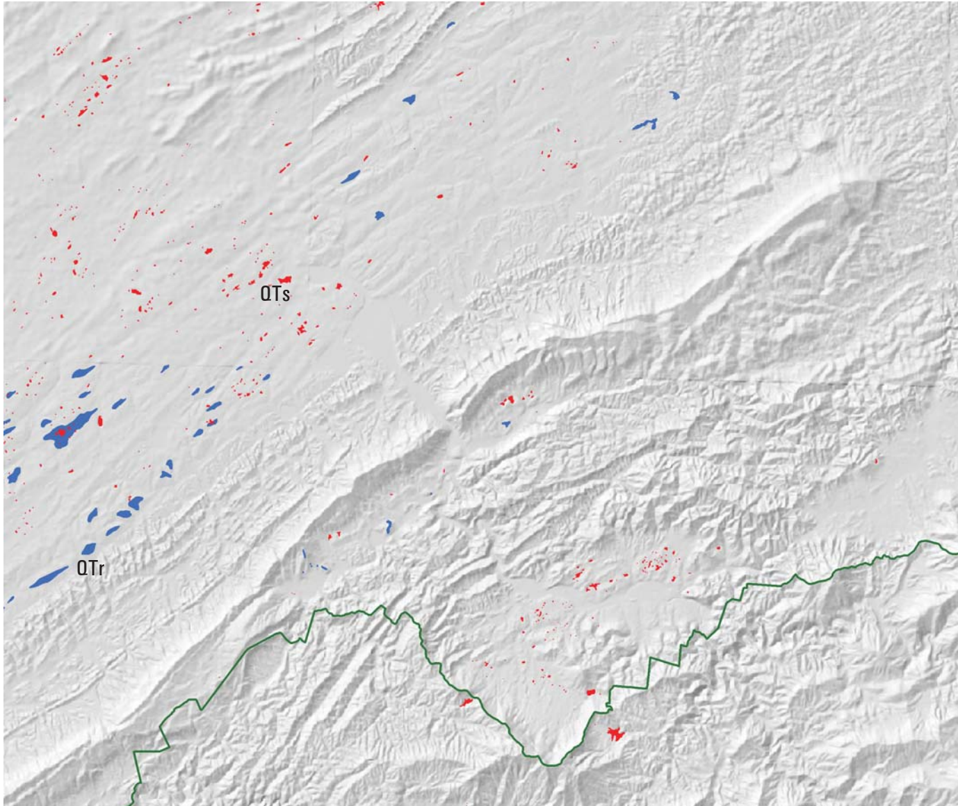
Fig. 22- Distribution of carbonate rocks and associated sinkholes (QTs, red) and residuum (QTr, blue) in the study area, shown on a digital elevation model hillshade.
