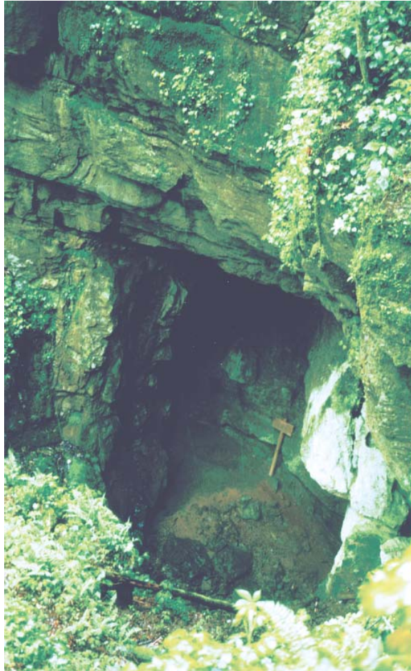
Fig. 24- Bull Cave on Rich Mountain is developed in Jonesboro Limestone (elevation 1900 ft, Kinzel Springs quadrangle).
