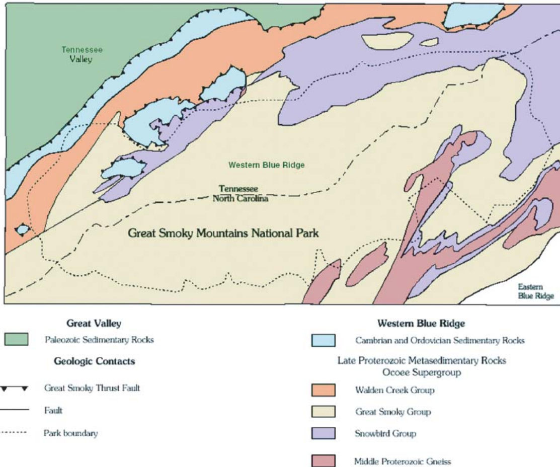
Fig. 3- Generalized geologic map of the study area, modified after Schultz and Southworth, 2000.
