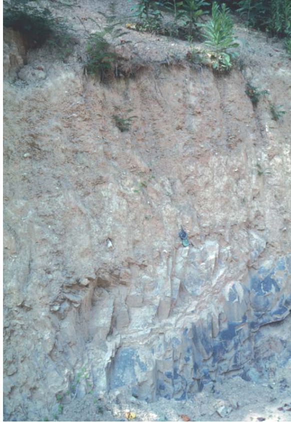
Fig. 30- Excavation, about 4m deep, showing residuum of Pigeon Siltstone overlain by colluvium of fine chips of siltstone, near Gatlinburg (elev = 1600 ft, Mt. Le Conte quadrangle).
