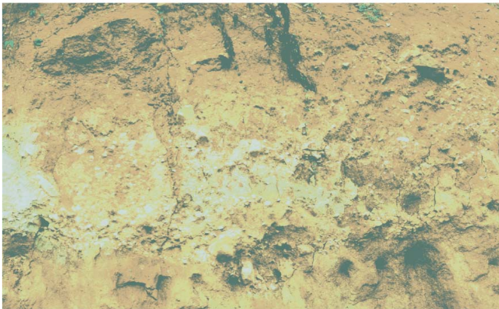
Fig. 31- B) Close-up showing residuum of sub-angular quartz gravel and oxidized soil derived from biotite gneiss (elev= 1960 ft, Whittier quadrangle).
