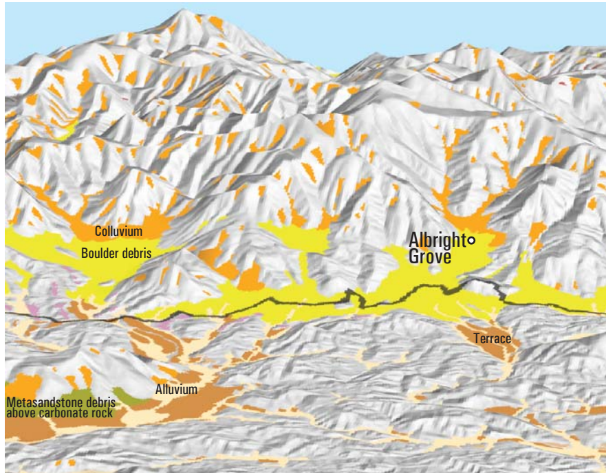
Fig. 55 -Isometric perspective of digital elevation model looking south at boulder debris fan of Dunn Creek in Albright Grove (Jones Cove and Mount Guyot quadrangles). This fan forms the drainage divide of two tributaries for 2 mi (3 km) that diverge at the base of the fan and enter the French Broad River 25 mi (40 km) apart.
