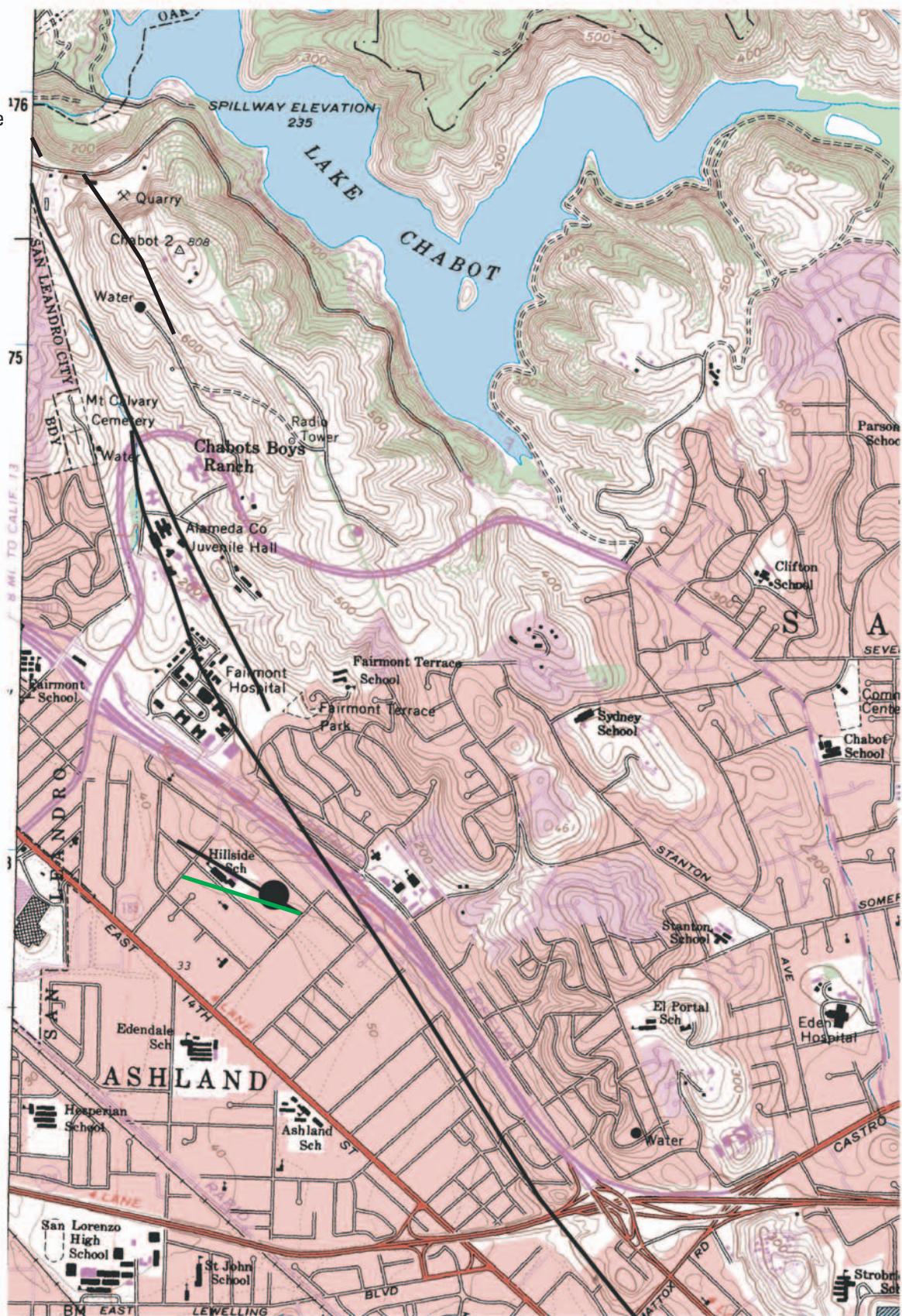
Figure 4-1. Topographic map the Ashland district of San Leandro. The mapped active strands of the Hayward Fault are shown as thick black lines, the active trace at fieldtrip stop 4 is shown as a thick green line, and the rough position of the trench site is shown as a black dot.
