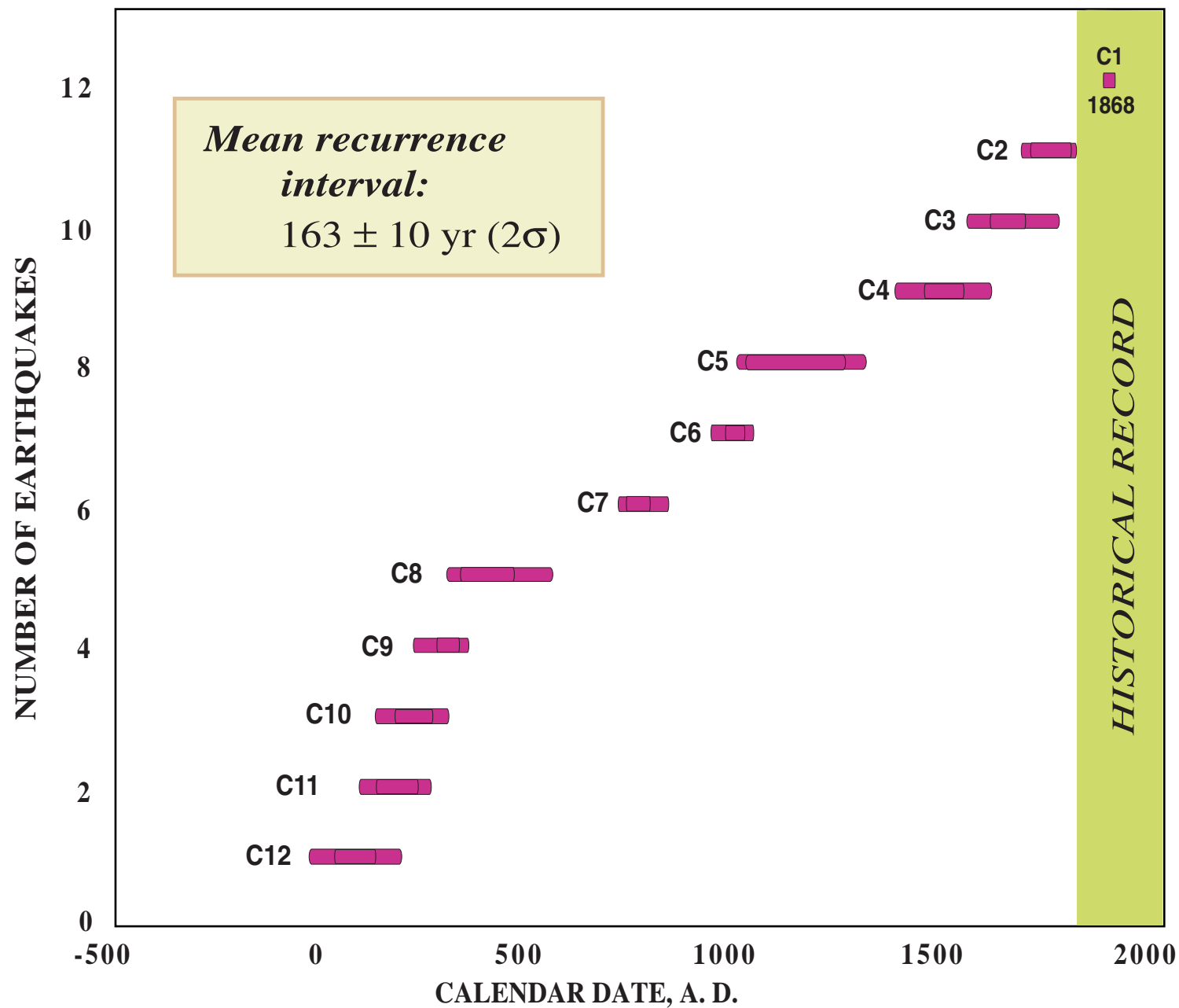
Figure 1-3. Preliminary 2000-year earthquake history on the southern Hayward Fault. The age of paleoearthquakes is shown as rounded pink rectangles (events C1 through C12) at 95-percentile uncertainty; darker pink shows 68-percentile confidence range. The age of the unit underlying event C12 is currently subject to ambiguity; an alternative age value gives mean recurrence of 173 \pm 10 \text{ yr} for events C1 through C11. Thus the mean recurrence interval for the last 2000 years can be stated as 168 \pm 15 \text{ yr (2}\sigma\text{)} while encompassing both interpretations. The plot above seems suggestive of periods of frequent earthquakes separated by quiescence, however, several more radiocarbon dates are needed to constrain actual variability within this sequence. Also, periods of slow sedimentation rate may allow 1-2 events to escape documentation, thus the mean recurrence interval discussed above may represent a minimum estimate.
