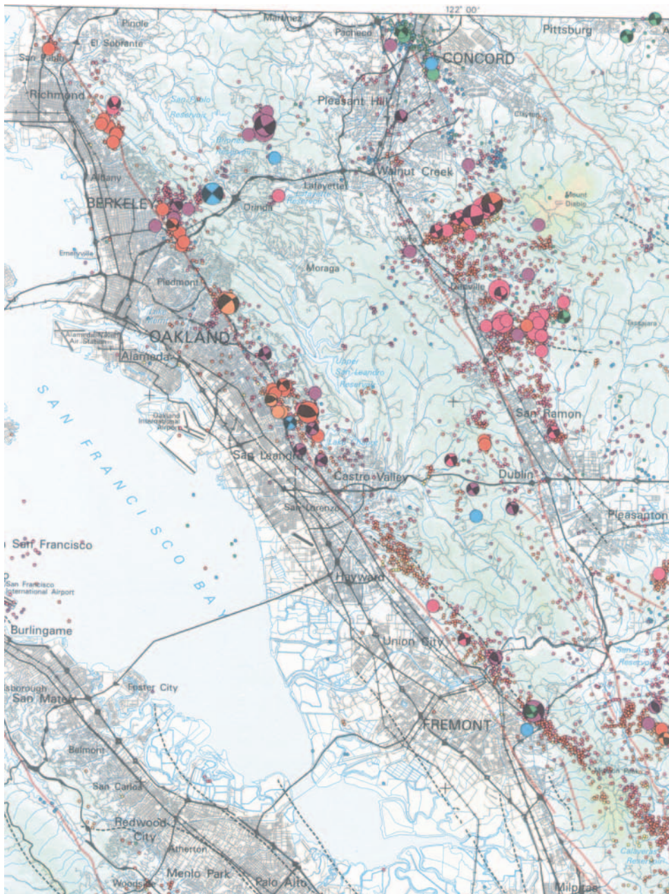
Figure 2-5. Seismicity in the east San Francisco Bay area (from Walter and others, 1998). Note the divergence of seismicity from the mapped active trace of the Hayward Fault southeast of Hayward, roughly along the trend of the Mission Fault. We now believe that this apparent divergence is related to hypocenters being deeper to the south along an east-dipping Hayward Fault, as well as shallower fault-plane dip in the left-step region of connection to the central Calaveras Fault.
