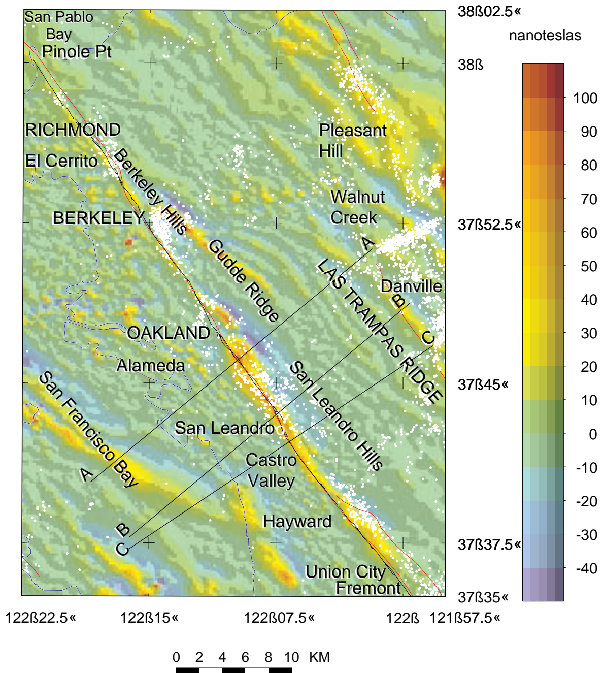
Figure 4-4. Magnetic map enhancing shallow magnetic sources along the Hayward Fault Zone. Shallow magnetic sources were enhanced by upward continuing the magnetic data a small distance (250 m) and then subtracting this field from the unfiltered data set to derive a residual field. The resulting map highlights magnetic sources within about 2.5 km of the surface. Red lines, faults from Jennings and others (1977); black line, recent trace of the Hayward fault from Lienkaemper (1992), white circles, seismicity data from the USGS's Northern California Seismic Net from September 1969 through September 1999, M greater than or equal to 1.0.
