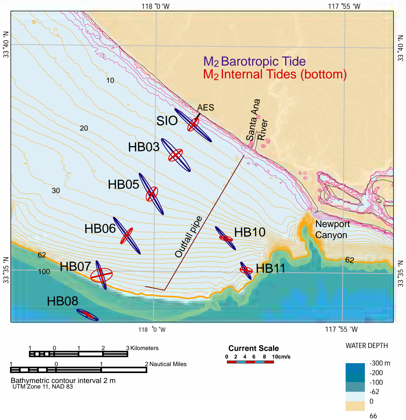
Figure 13. M 2 tidal current ellipses for barotropic and baroclinic tides at the bed. The strongest tidal currents flow parallel to the long axis of the ellipse.
