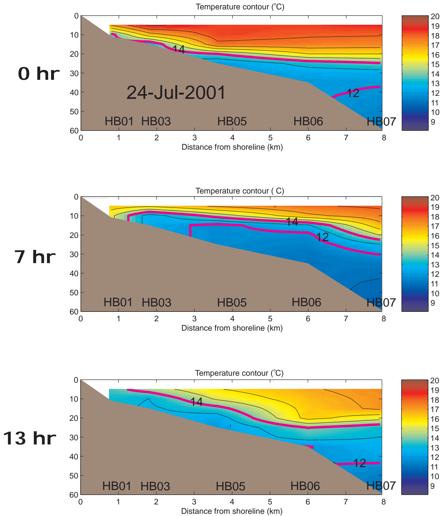
Figure 15. Temperature profiles for the rising, peak and falling portion of a cold pulse event on July 24.
