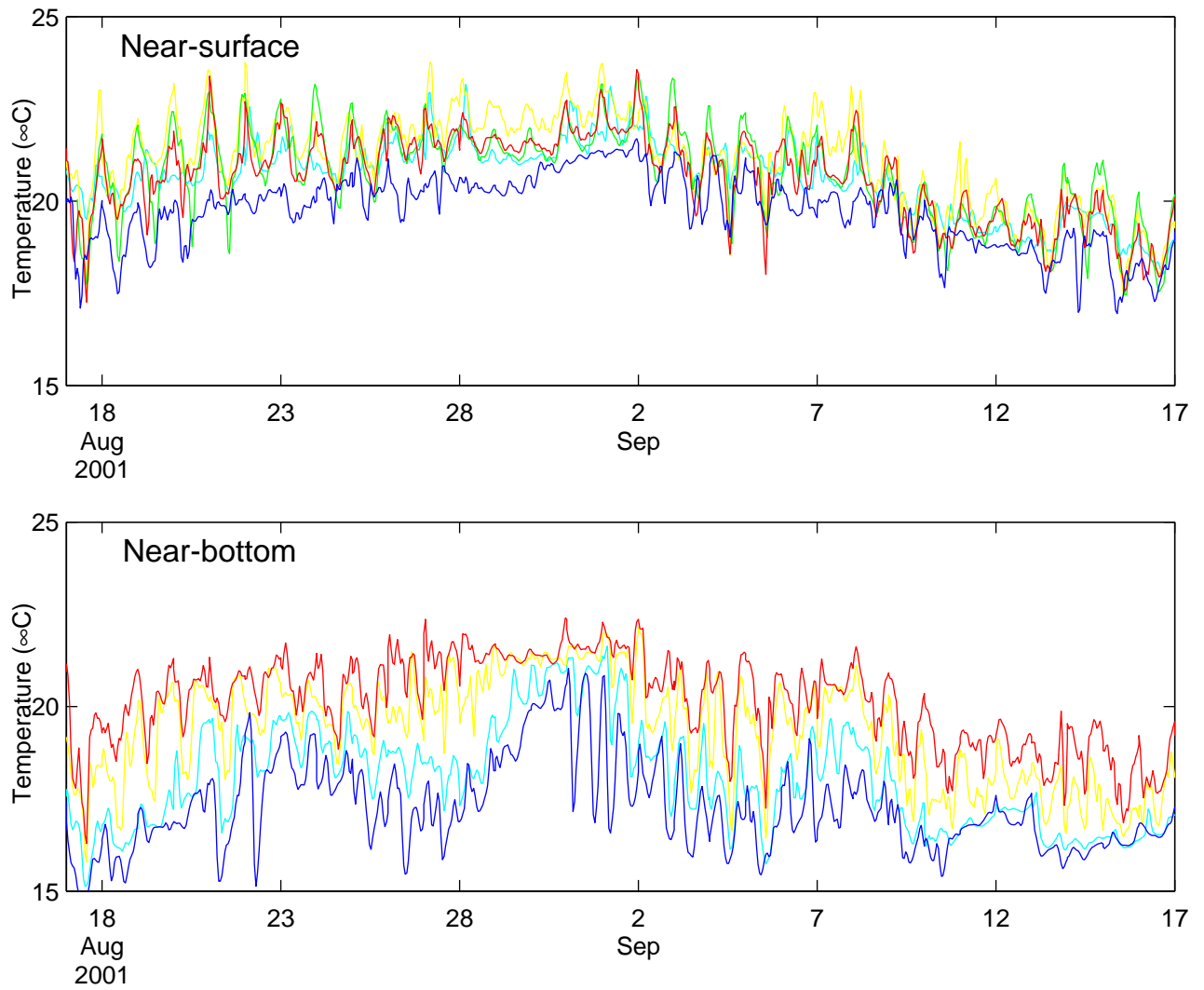
Figure 16. Temporal variations in near-surface and near-bottom temperatures at mooring in 15m (blue), 10m (turquoise), 7.5m (yellow), 2.5m (red), and 0.5m (green).
