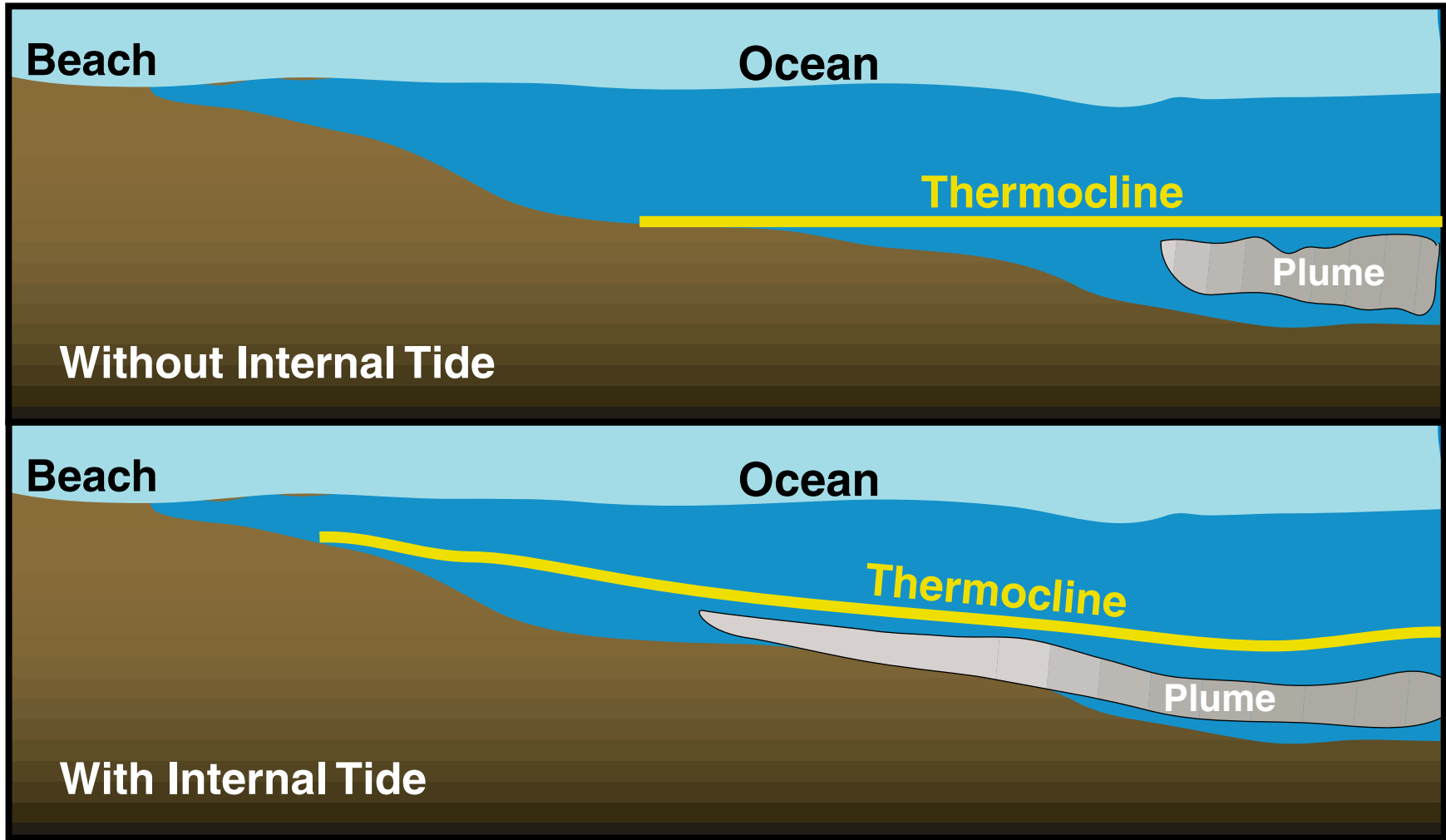
Figure 2. Schematic of cross-shore transport of the plume from the outfall by internal tidal currents.
