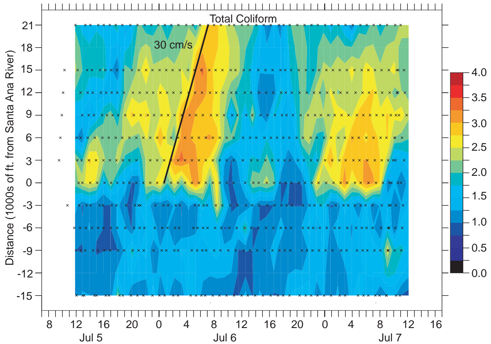
Figure 6. The log 10 of total coliform concentration (mpn/100 ml) is plotted versus local time and distance alongshore. Black x's indicate the time and location of each sample.
