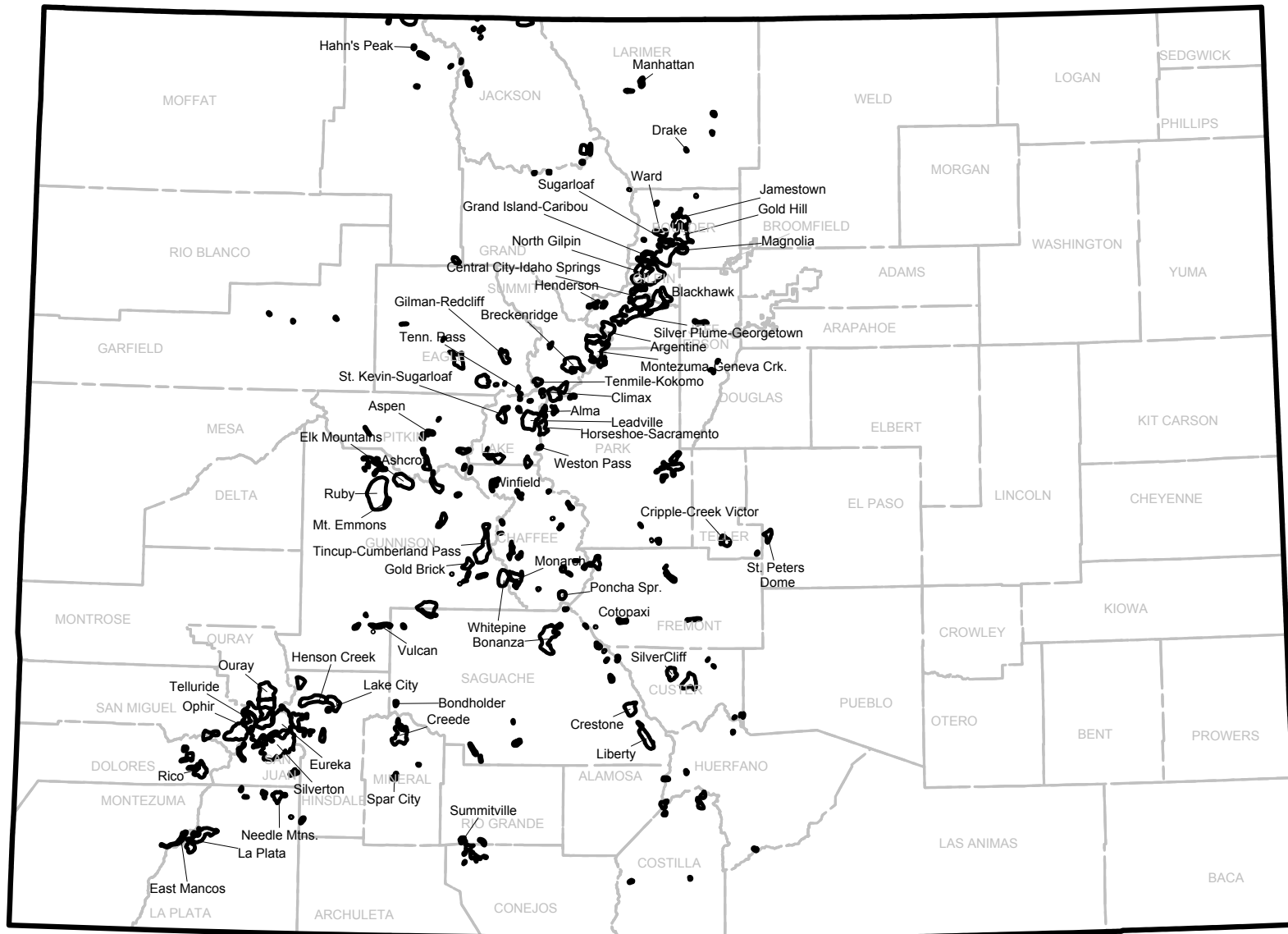
Generalized map showing mineralized areas in Colorado
