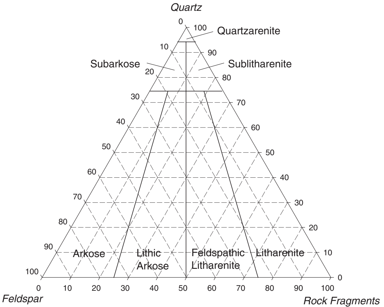
Figure 1. Ternary diagram showing sandstone classification nomenclature.
