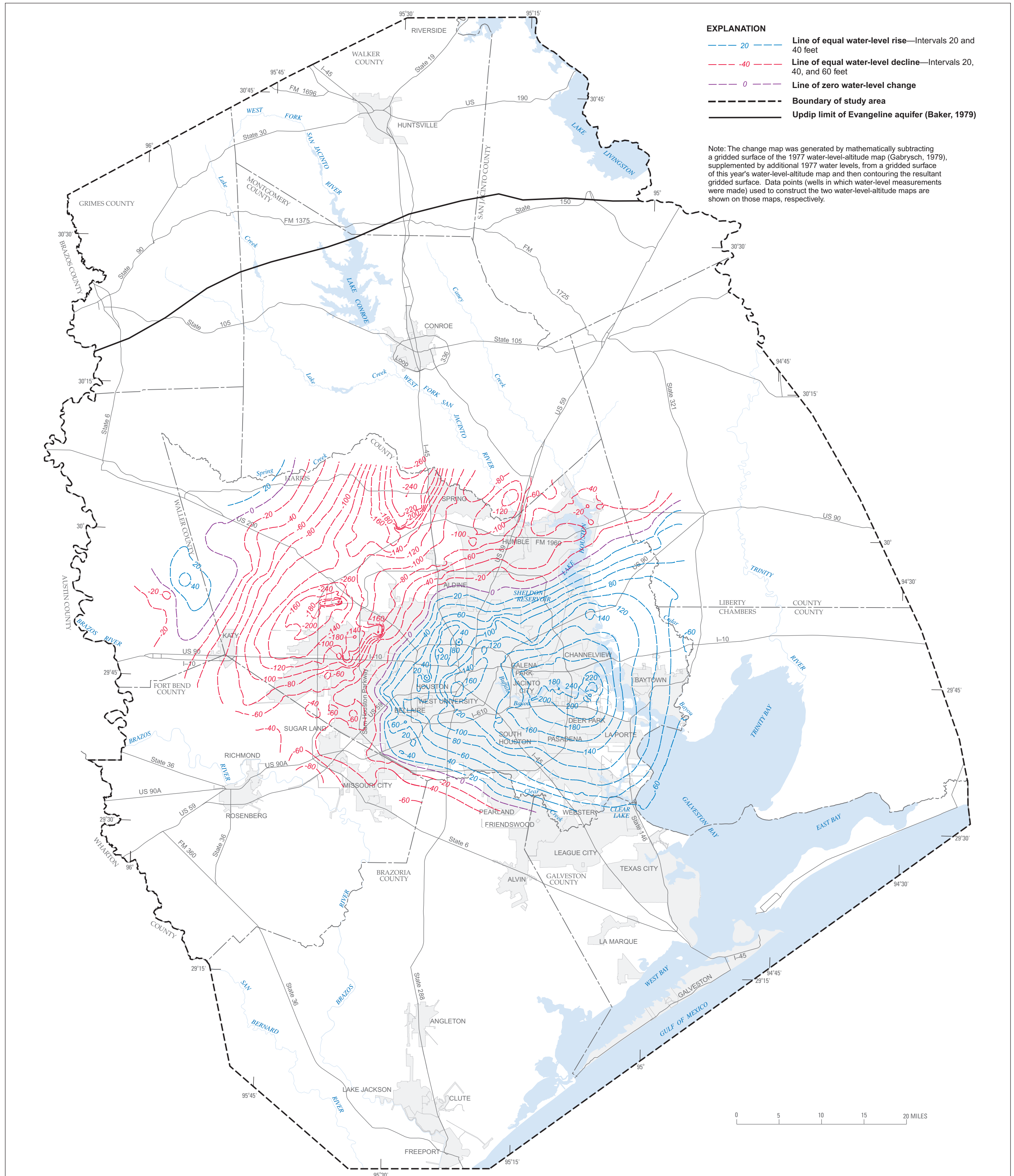
Figure 9. Map showing approximate water-level changes in the Evangeline aquifer, Houston-Galveston region, Texas, 1977-2003.
