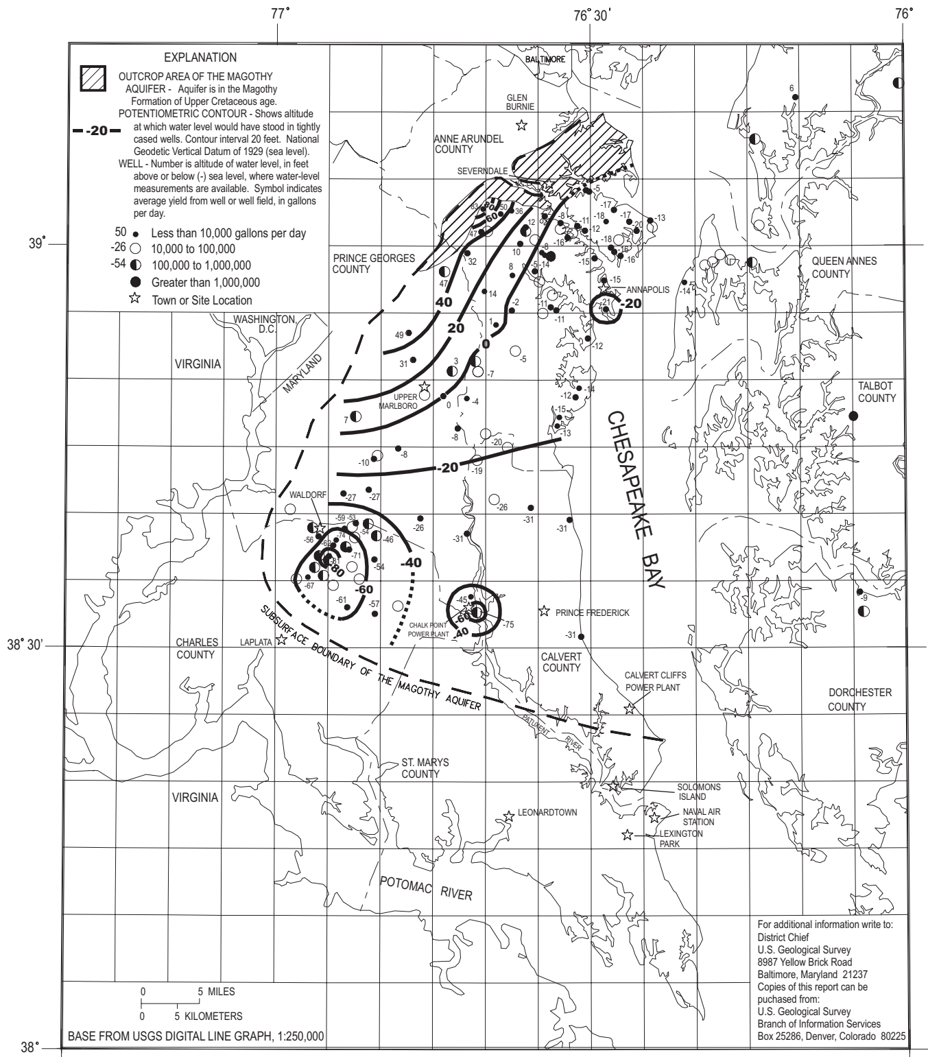
POTENTIOMETRIC SURFACE OF THE MAGOTHY AQUIFER IN SOUTHERN MARYLAND, SEPTEMBER 2002
