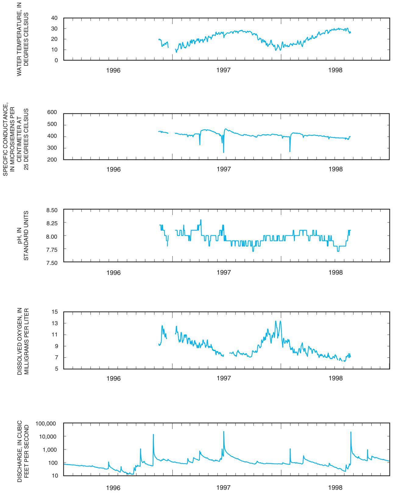
Figure 6. Daily mean water temperature, specific conductance, pH, dissolved oxygen, and stream discharge for Frio River at Concan, Texas (08195000), January 1996–December 1998.
