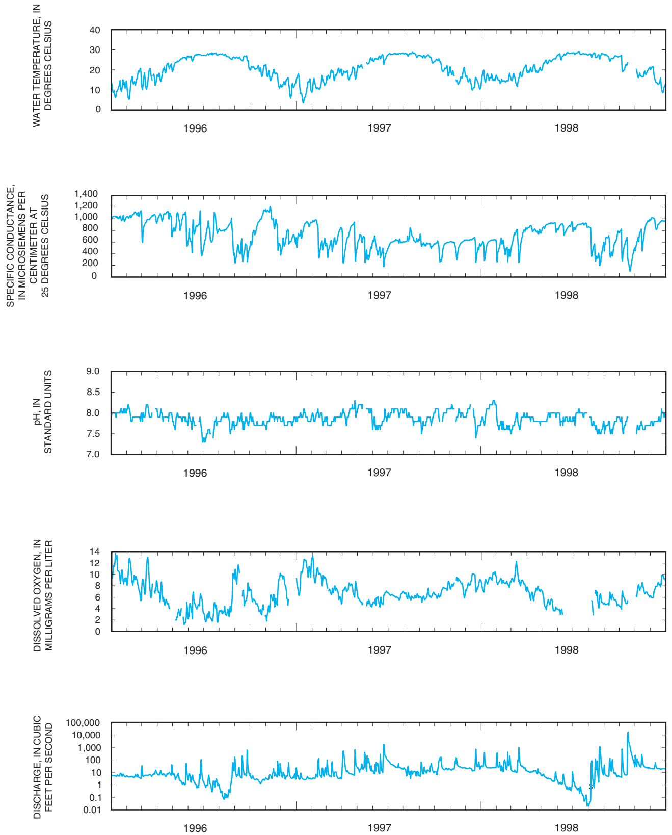
Figure 10. Daily mean water temperature, specific conductance, pH, dissolved oxygen, and stream discharge for Salado Creek (lower station) at San Antonio, Texas (08178800), January 1996–December 1998.
