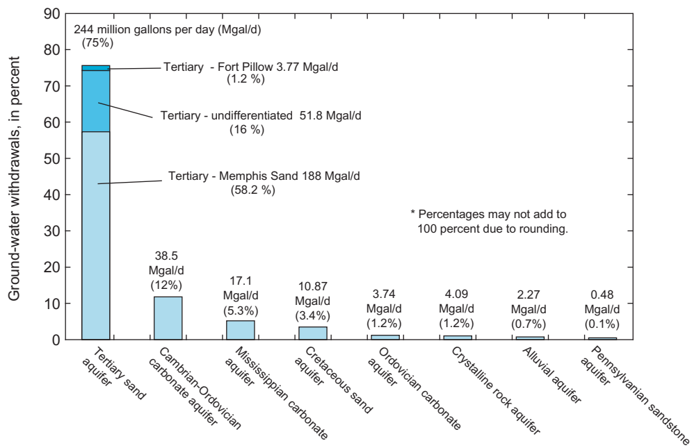
Figure 4. Ground-water withdrawals from principal aquifers in Tennessee, 2000.
