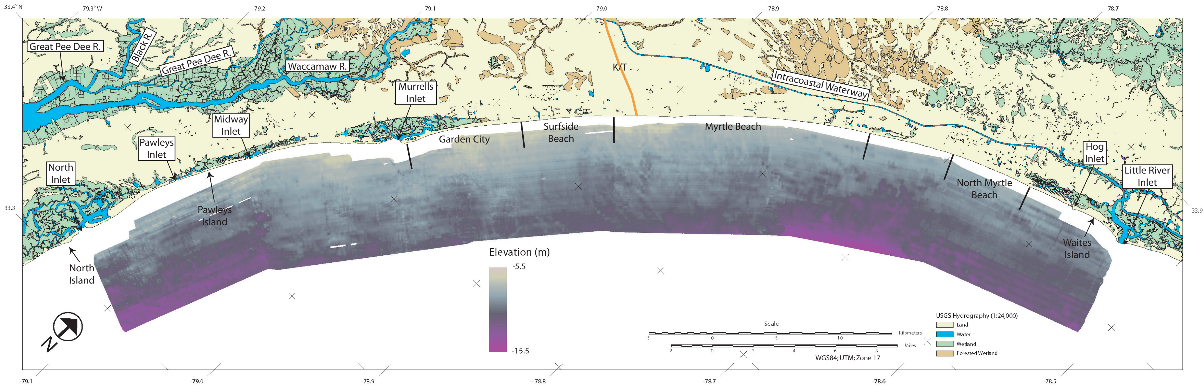
Figure 16. Elevation of regionally defined transgressive surface as mapped from CHIRP sub-bottom profiles.
