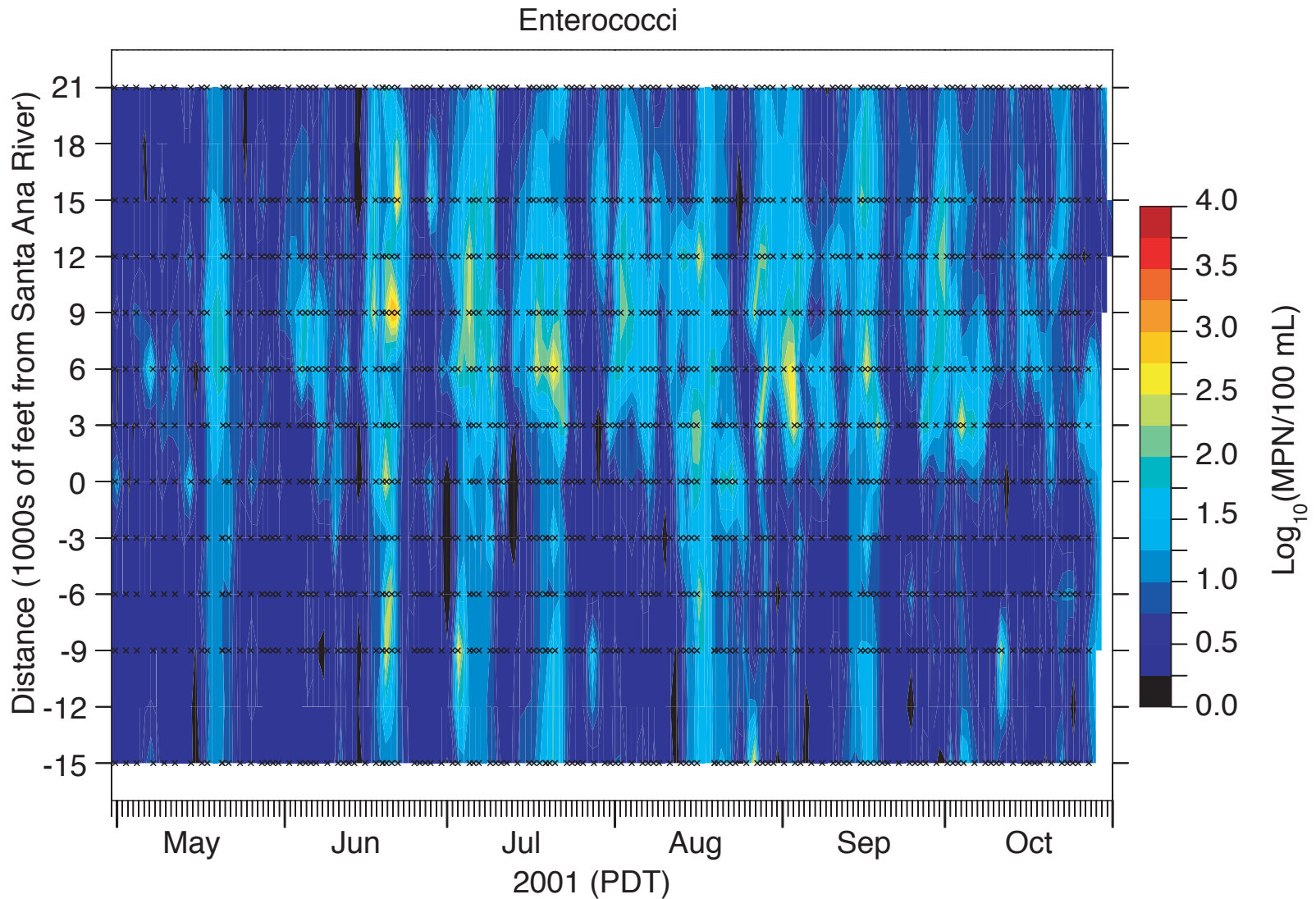
Figure 3-12. \text{Log}_{10} of enterococci concentration (MPN/100 mL) is plotted versus time and distance alongshore. The data set subsampled to no more than daily values was used. X's indicate the day and location of each sample. Data is contoured with PlotPlus on a 180 x 13 grid (time and distance, respectively) using cay=5 and nrng=2. The cay value determines the interpolation scheme. Cay=0 means Laplacian interpolation is used. As cay is increased, spline interpolation predominates over Laplacian. For pure spline interpolation cay=infinity. Grid points are set to "undefined", and not used, if farther than nrng away from the nearest data point.
