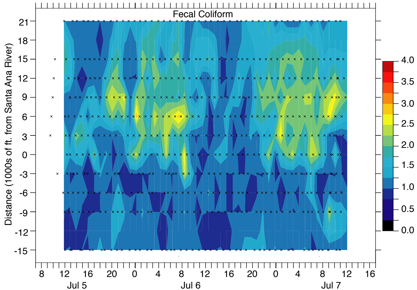
Figure 3-19. The \log_{10} of fecal coliform concentration (MPN/100 mL) is plotted versus local time and distance alongshore. Black x's indicate the time and location of each sample. Data is contoured on a 48 by 13 grid (time and distance, respectively) using cay=5 and nrrng=2 . Time is Pacific Daylight Time (PDT).
