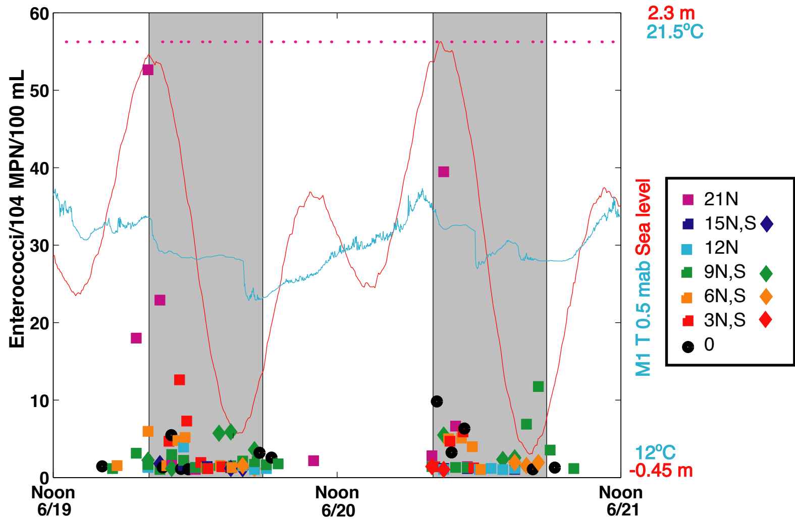
Figure 3-29. The ratio of enterococci concentrations to the AB411 single-sample standard at stations 15S to 21N for the second intensive sampling period is plotted together with sampling times at station 0 (pink dots), Los Angeles sea level (red line), and temperature 0.5 m above bottom at HB01 (blue line). Only samples exceeding 104 MPN/100 mL are shown here. A local time reference is used.
