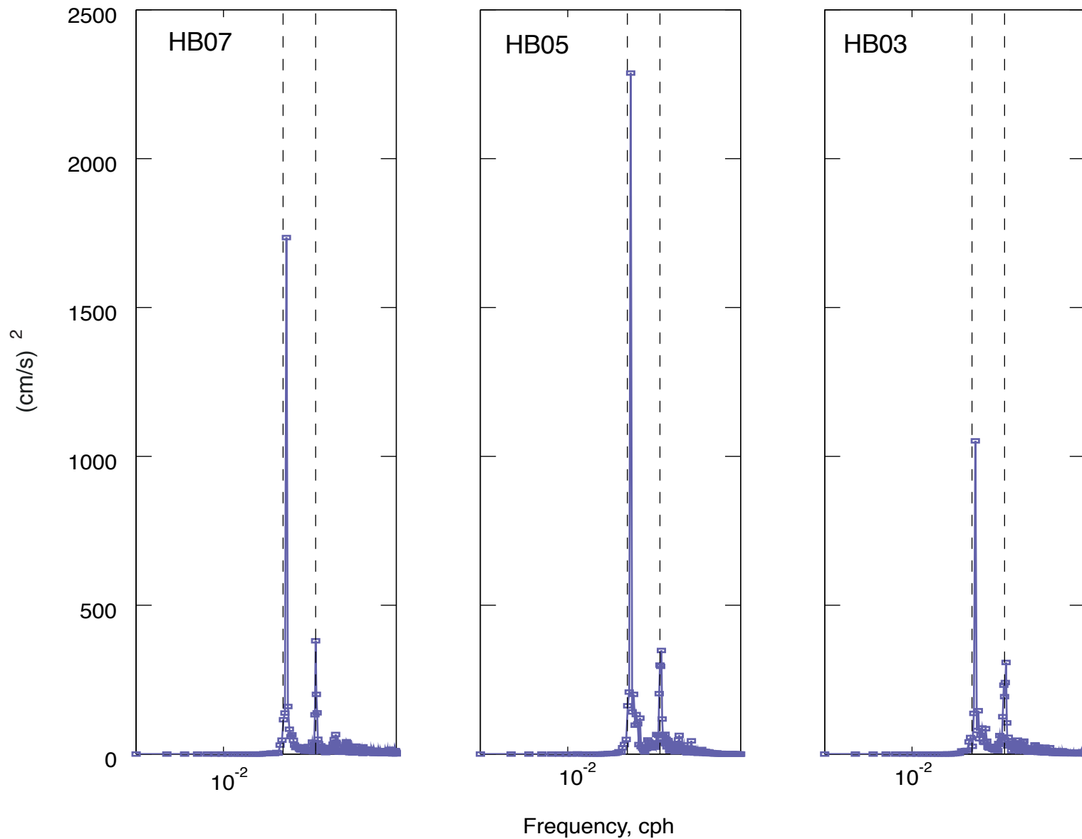
Figure 7-5b. Same as for Figure 7-5a, but for near-surface, alongshore data.
