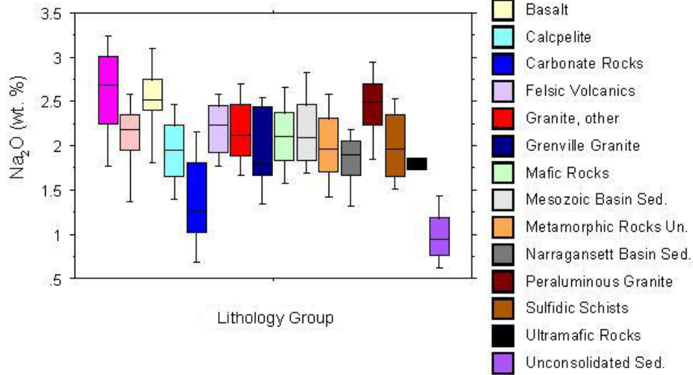
Values of Na 2 O, by Bedrock Lithology in New England
