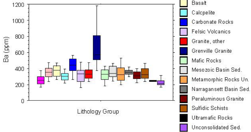
Values of Ba, by Bedrock Lithology in New England
