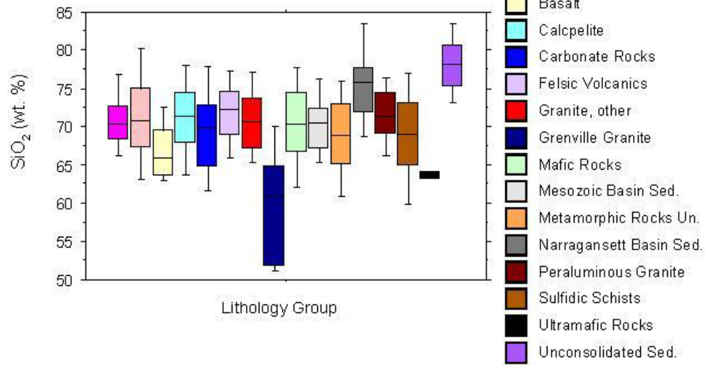
Values of SiO 2 , by Bedrock Lithology in New England
