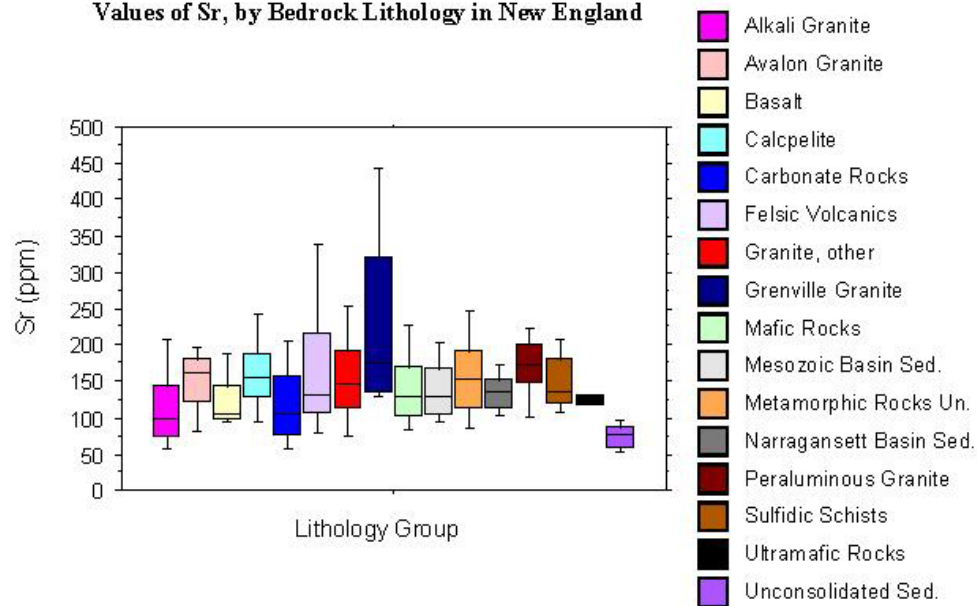
Values of Sr, by Bedrock Lithology in New England
