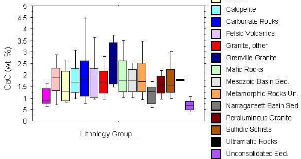
Values of CaO, by Bedrock Lithology in New England
