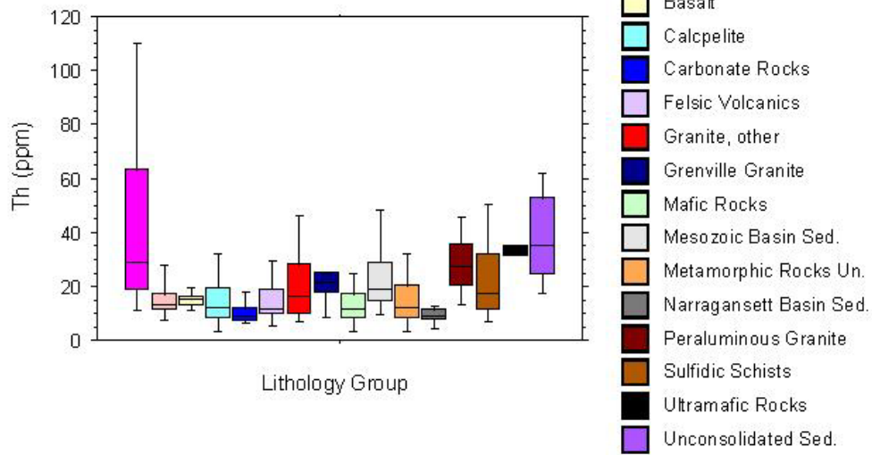
Values of Th, by Bedrock Lithology in New England
