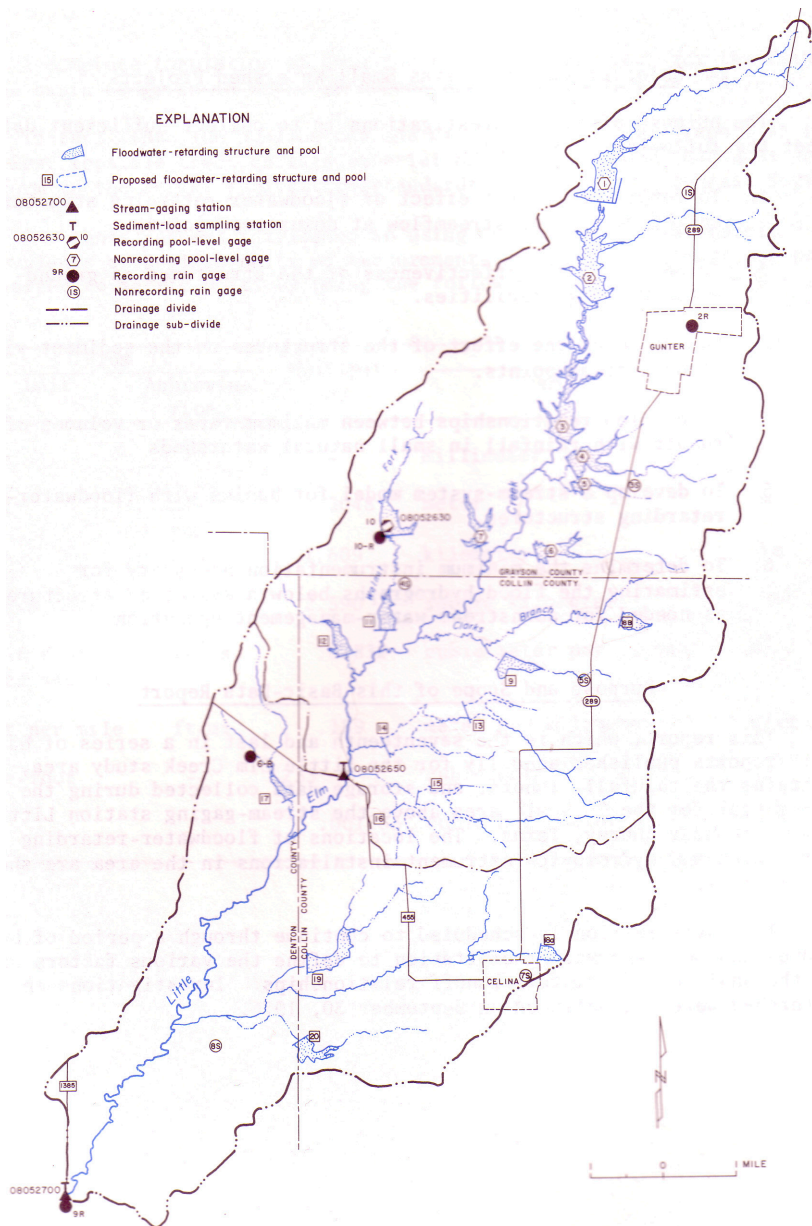
Figure 27. Location map for small rural watersheds database module for Little Elm Creek watershed adopted from Slade and Taylor, 1978.
