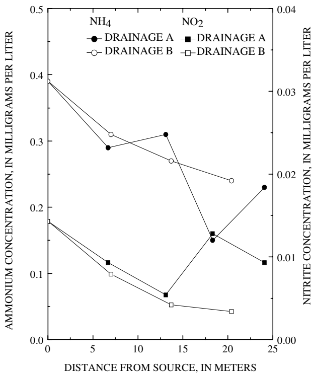
Figure 21. Sample pH, temperature, and concentrations of As(T), As(III), NH 4 and NO 2 as a function of drainage distance for Ojo Caliente Spring.
