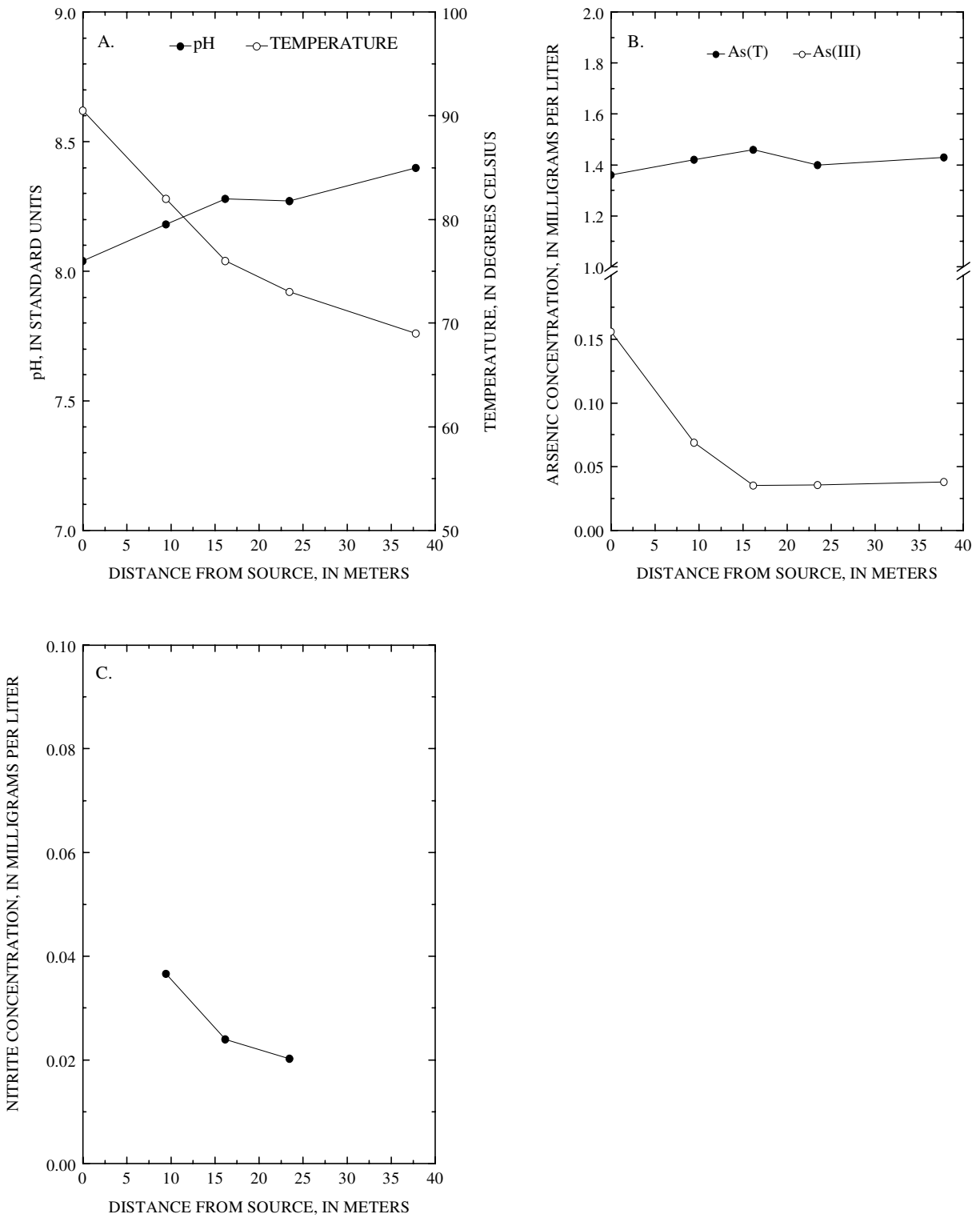
Figure 20. Sample pH, temperature, and concentrations of As(T), As(III), and NO 2 as a function of drainage distance for Octopus Spring.
