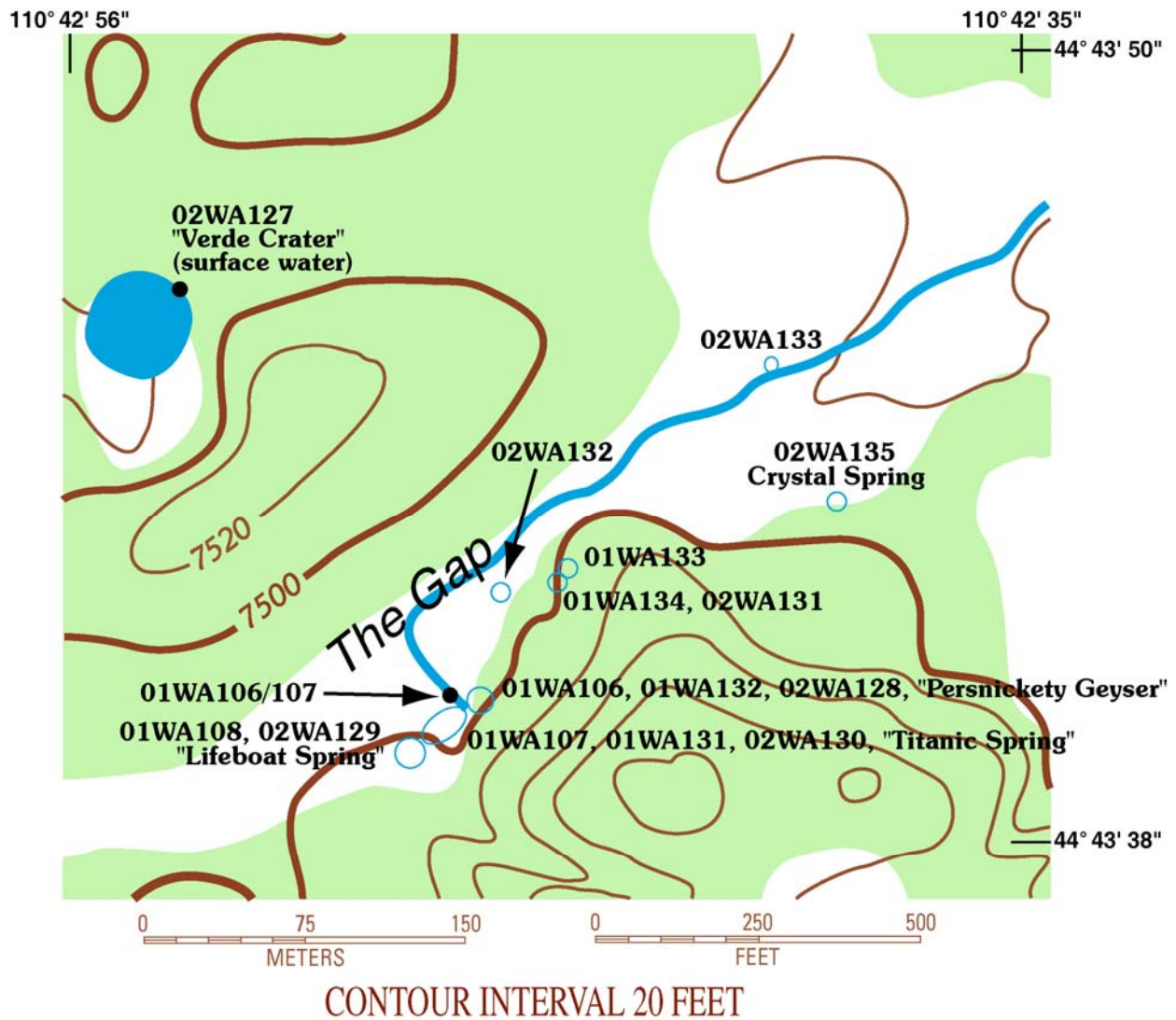
Figure 7. Sampling locations with sample code numbers for hot springs and one surface water sample in the Ragged Hills area of Norris Geysers Basin, Yellowstone National Park, Wyoming (see figure 4).
