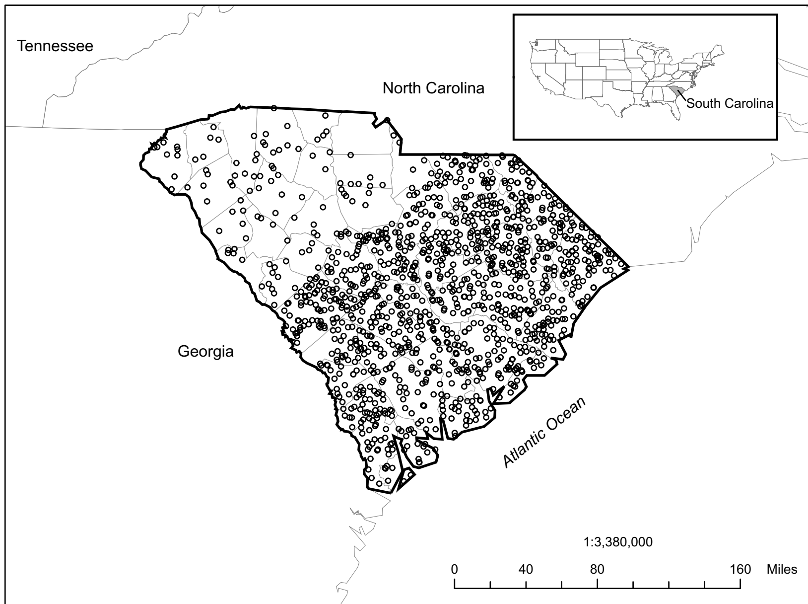
Figure 1. Locations of re-analyzed NURE stream-sediment samples in South Carolina (U.S. Geological Survey, 2004)
