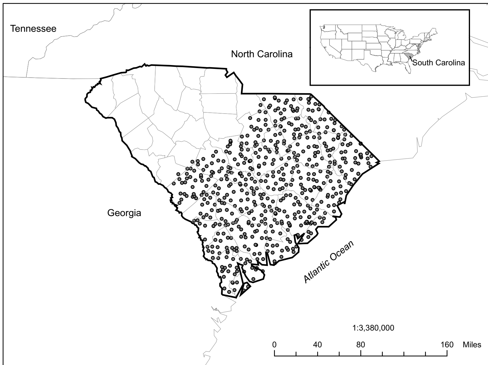
Figure 2. Locations of NGS soil samples in South Carolina (U.S. Geological Survey, 2004)
