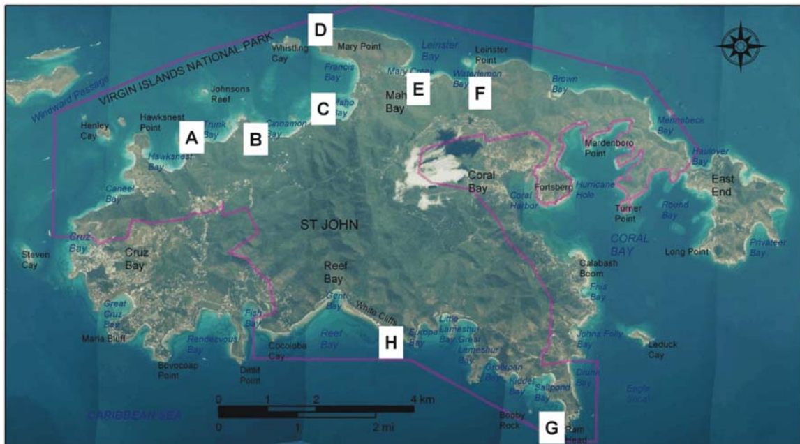
Figure 5. Photos of different geomorphologic types within Virgin Islands National Park. Click on a letter to see a photo near that location.
