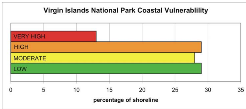
Figure 12. Percentage of Virgin Islands shoreline in each CVI category.
