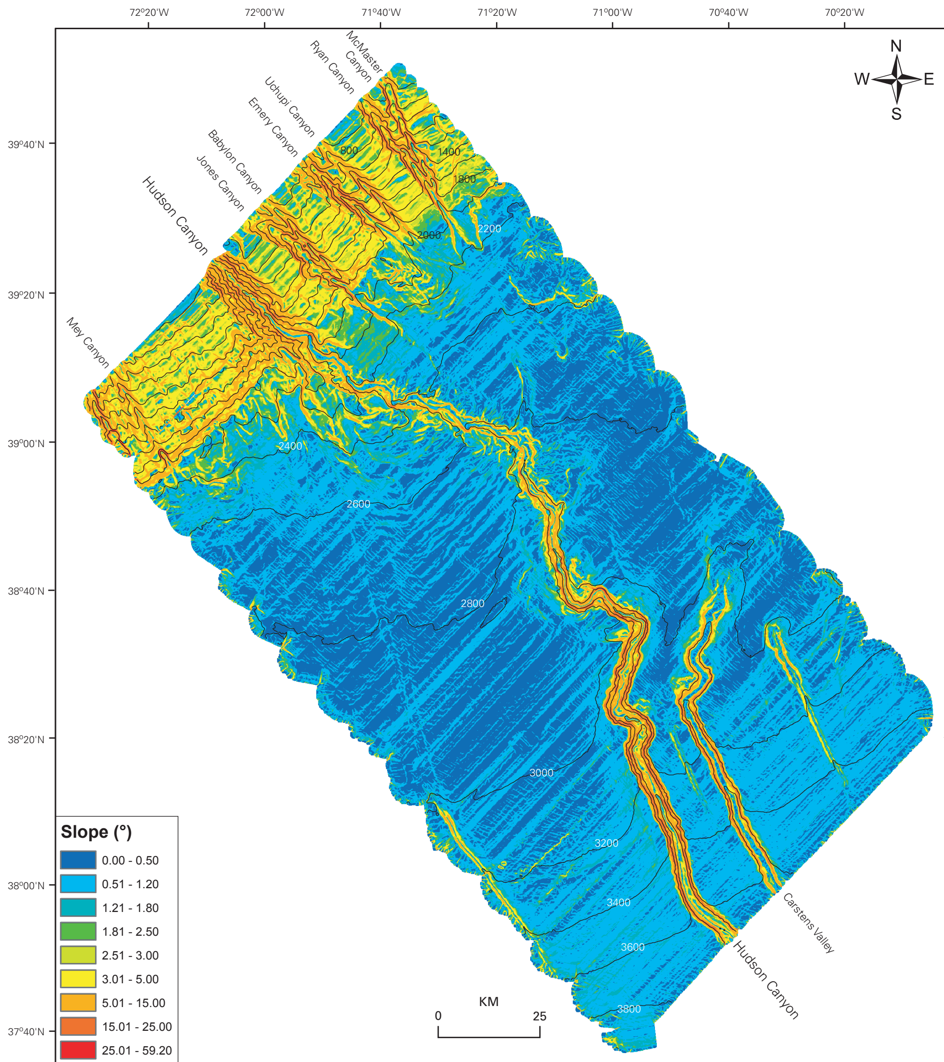
Figure 5. Map showing slope of the sea floor. The slope is typically 3-5° over the continental slope, less than 0.5 ° over the upper rise, and 0.5-1.2° over the lower rise. The slope of the canyon walls range from 5-25°.
