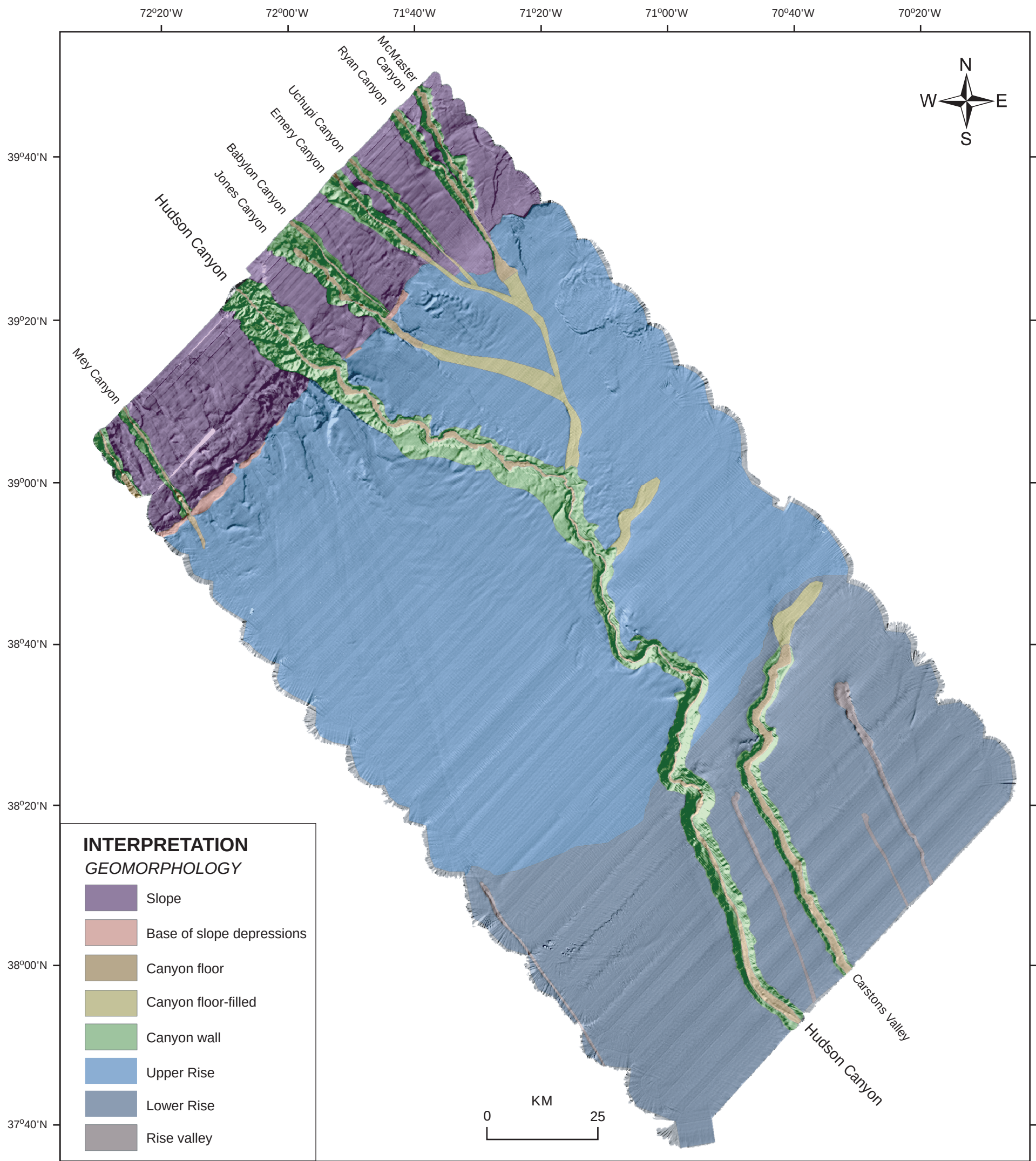
Figure 7. Geomorphic provinces identified in the study area.
