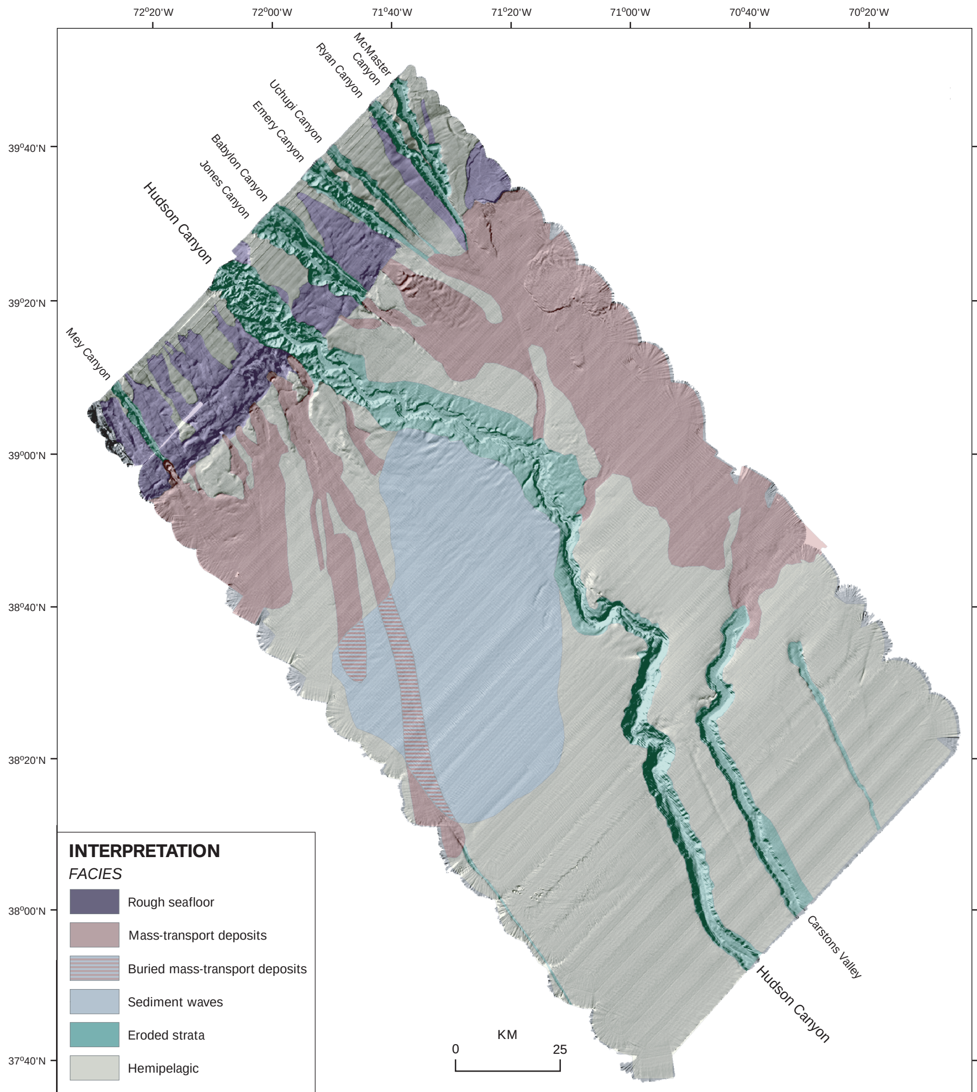
Figure 8. Map of sea-floor environments based on backscatter intensity and subbottom characteristics revealed in widely spaced 3.5-kHz subbottom profiles.
