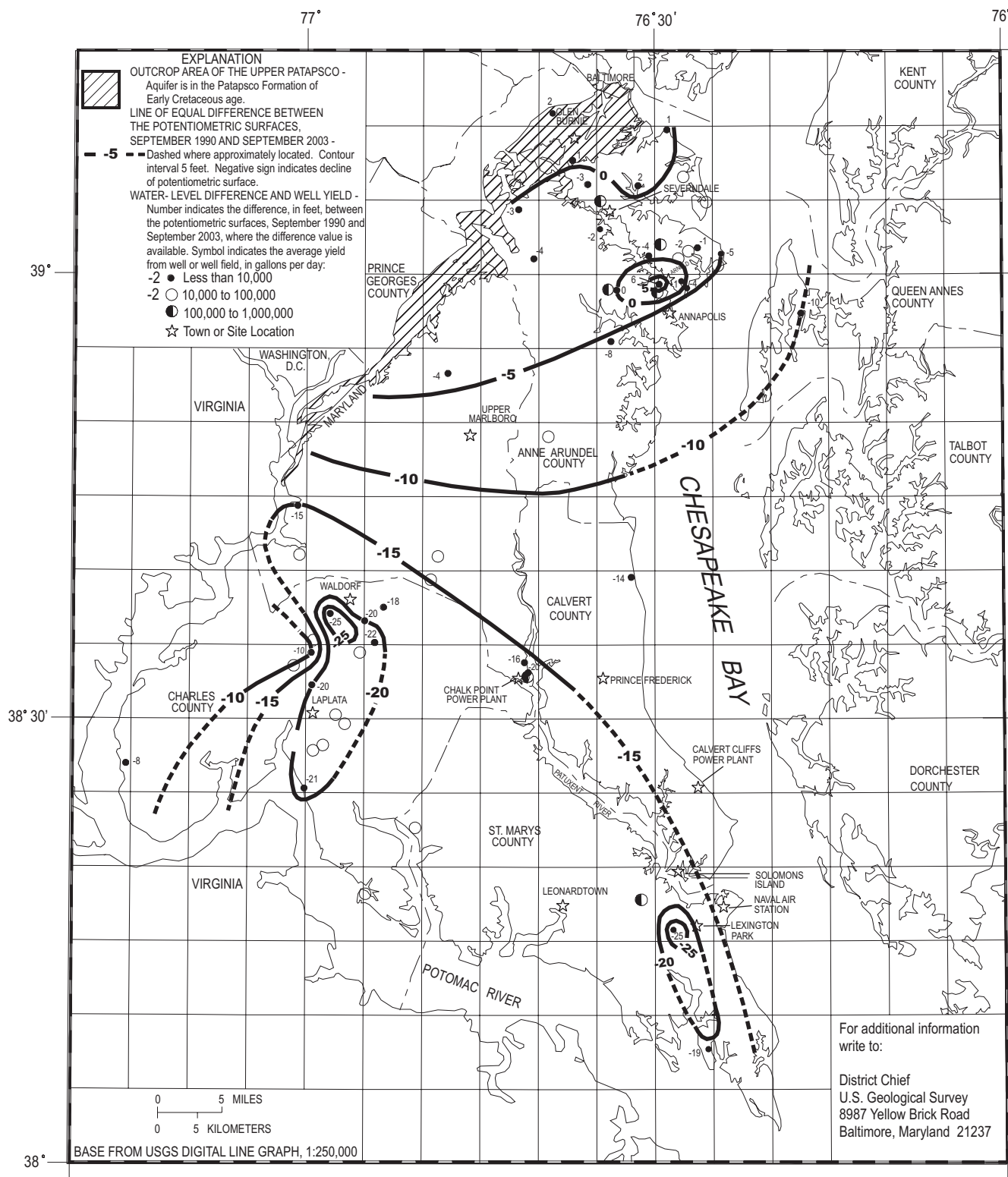
THE DIFFERENCE BETWEEN THE POTENTIOMETRIC SURFACES OF THE UPPER PATAPSCO AQUIFER, SEPTEMBER 1990 AND SEPTEMBER 2003 IN SOUTHERN MARYLAND
