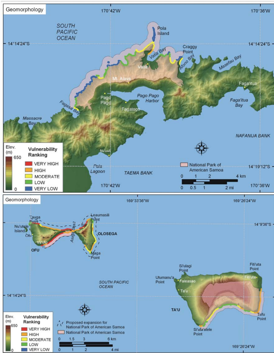
Figure 7. Vulnerability ranking for coastal geomorphology within the National Park of American Samoa. The colored shoreline represents the variations in coastal geomorphology within the park. The National Park of American Samoa consists of several geomorphology types, including very high vulnerability carbonate sand beaches, high vulnerability rubble to cobble shoreline skirted by fringing reef, moderate vulnerability alluvium and narrow fringing reef with cliffs, and low and very low vulnerability rock cliffs.
