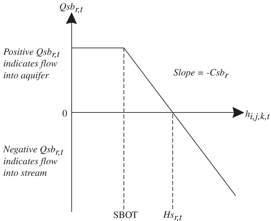
Figure 1. Seepage rate, Q_{sb_{r,t}} , through a streambed as a function of ground-water head, h_{i,j,k,t} , in a model cell, where SBOT is the streambed bottom, Csb_r is streambed conductance, and Hs_{r,t} is head in the stream. Figure modified from Prudic (1989).
