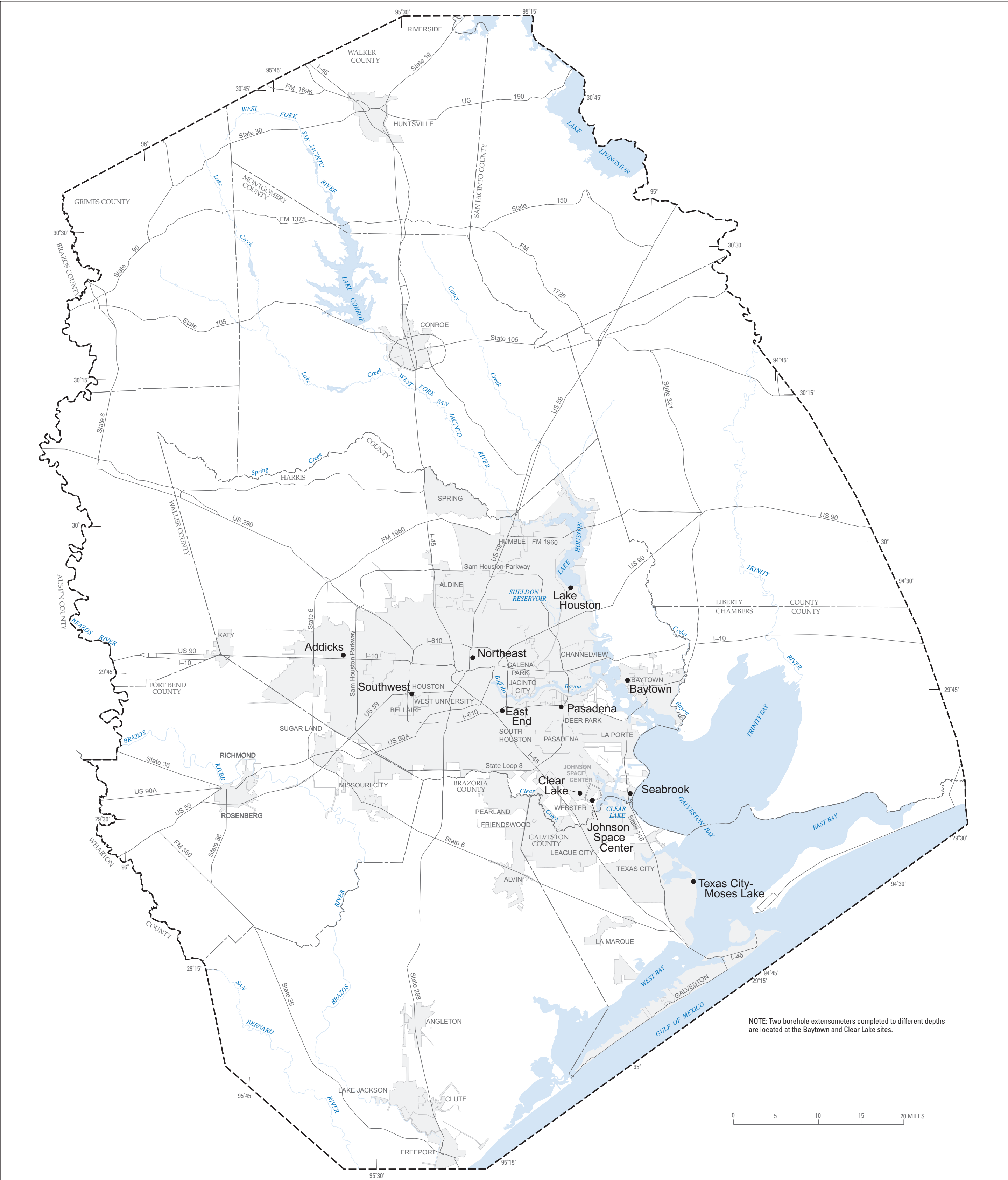
Figure 14. Map showing location of borehole extensometer sites, Houston-Galveston region, Texas.
