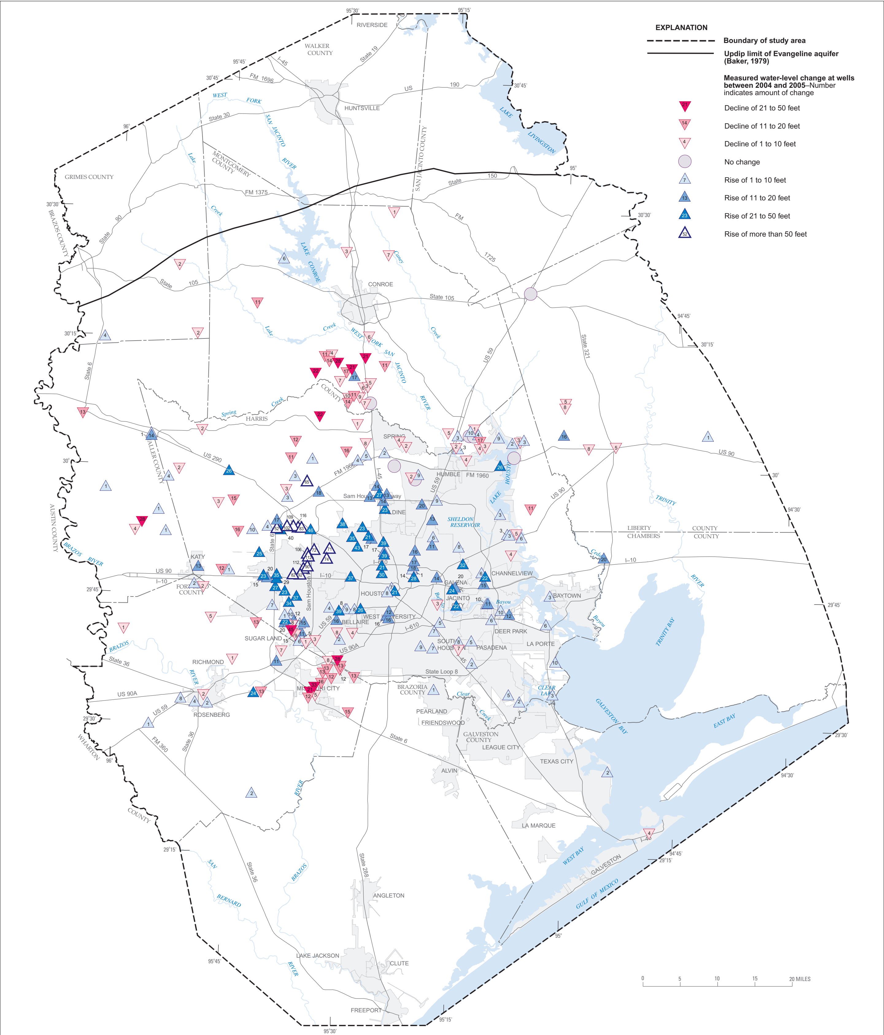
Figure 7. Map showing water-level changes in the Evangeline aquifer, Houston-Galveston region, Texas, 2004-05.
