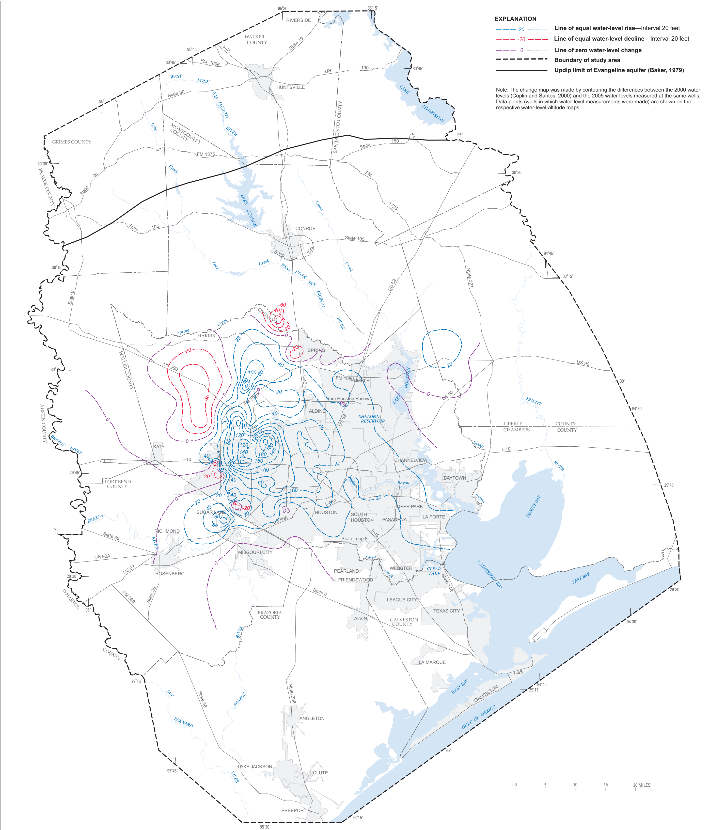
Figure 8. Map showing approximate water-level changes in the Evangeline aquifer, Houston-Galveston region, Texas, 2000-2005.
