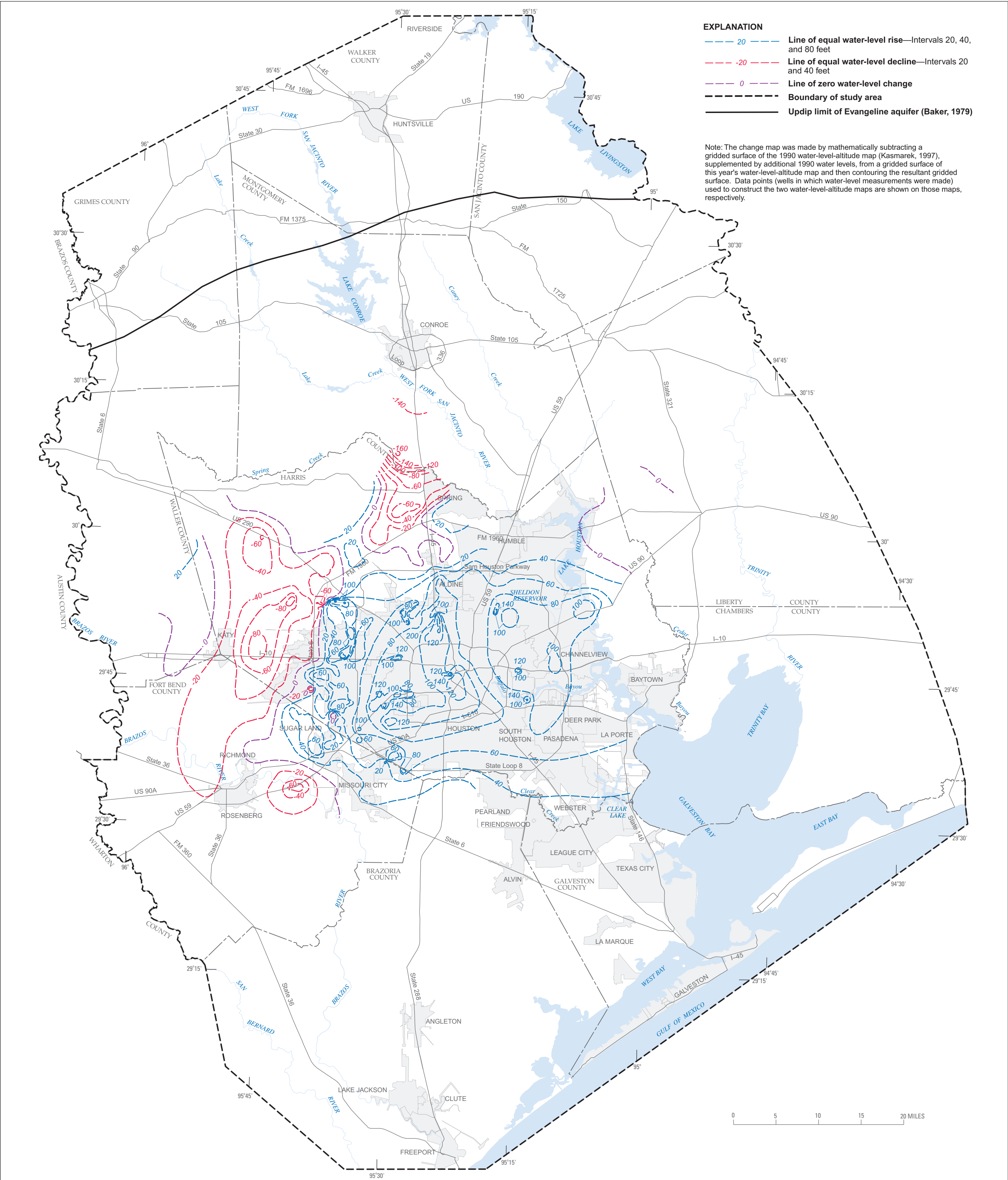
Figure 9. Map showing approximate water-level changes in the Evangeline aquifer, Houston-Galveston region, Texas, 1990-2005.
