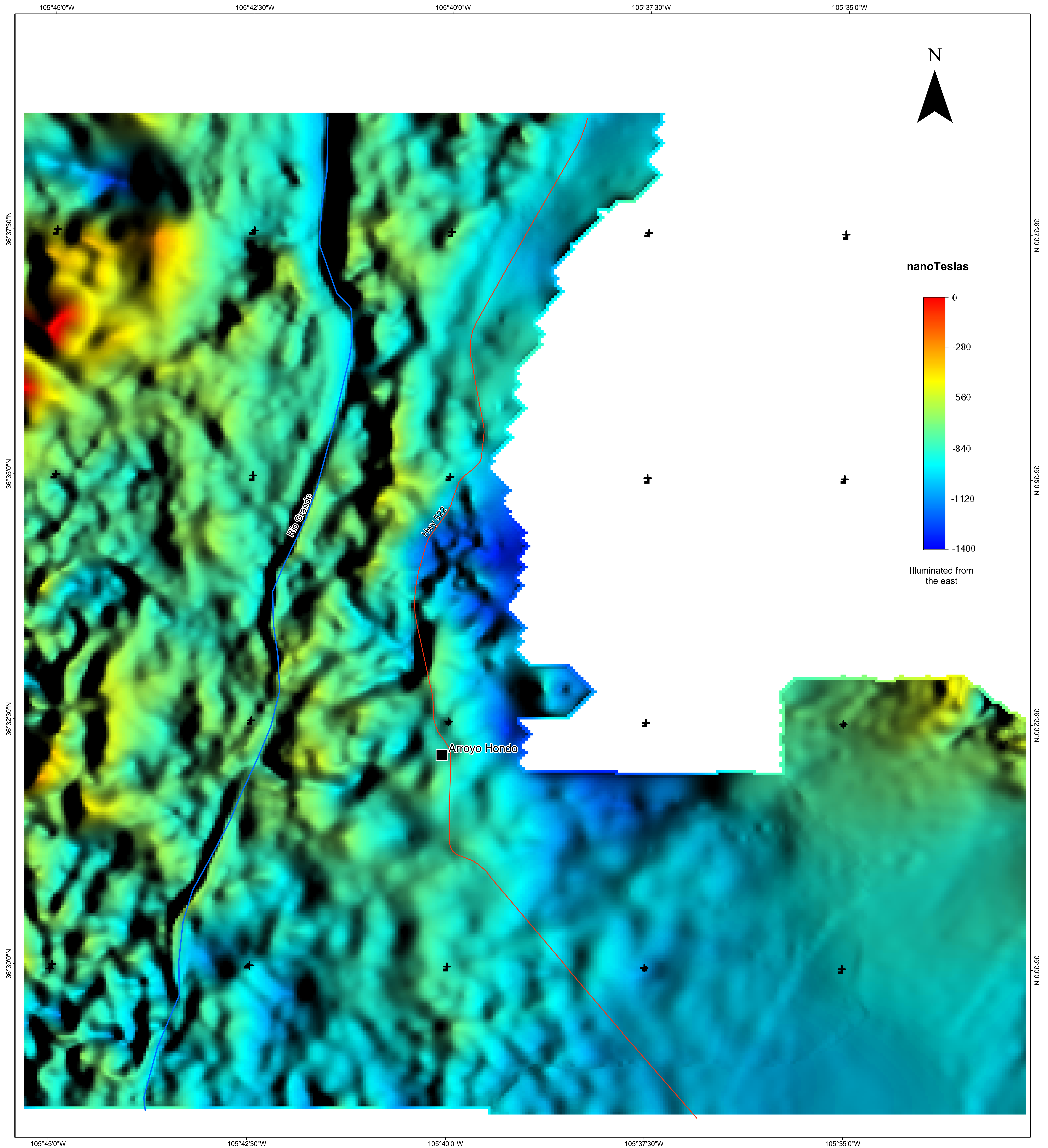
Central San Luis Basin Aeromagnetic Survey Color shaded-relief image of continued, reduced-to-pole (RTP) magnetic data, Arroyo Hondo area.
