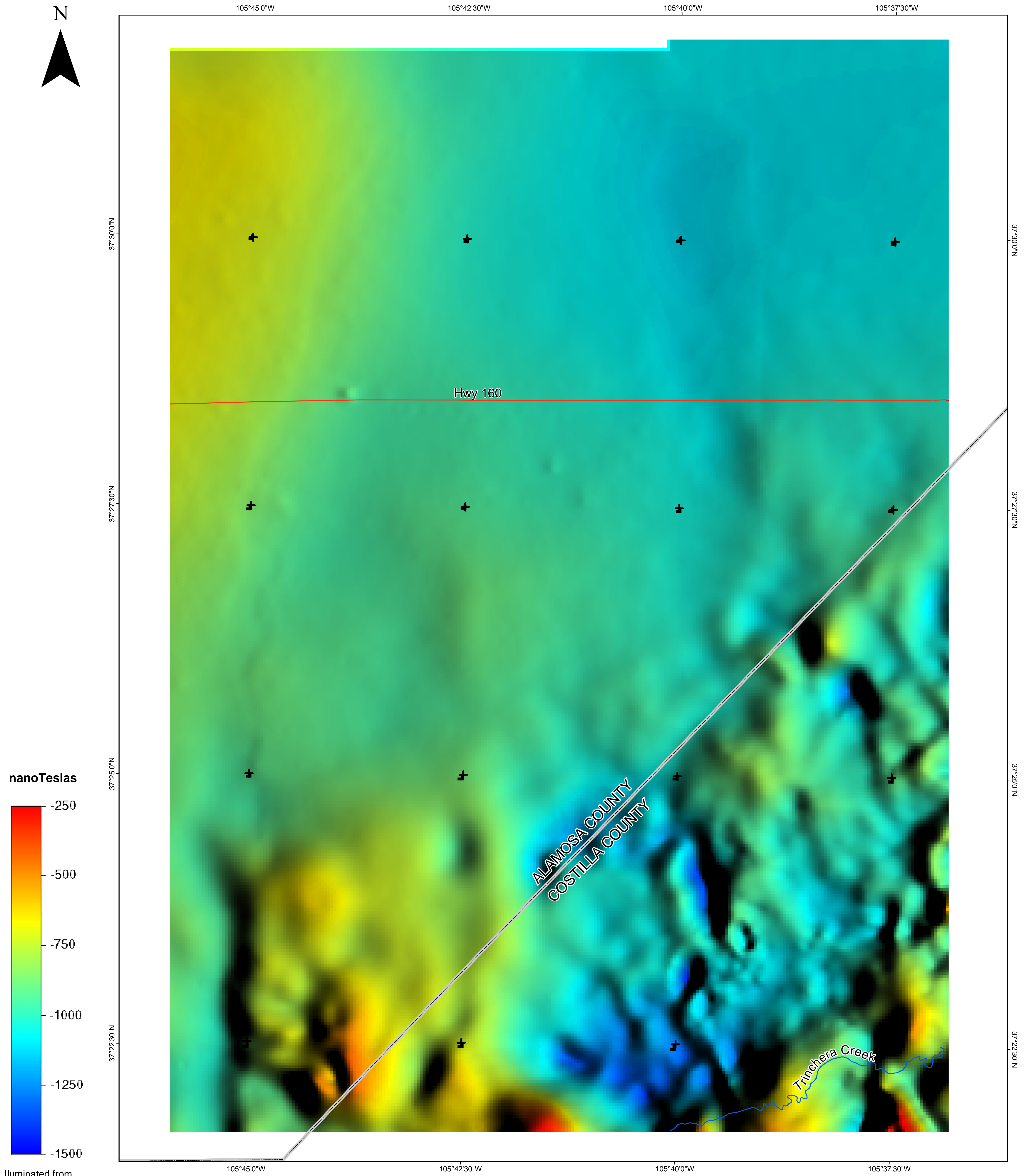
Central San Luis Basin Aeromagnetic Survey Color shaded-relief image of continued, reduced-to-pole (RTP) magnetic data, Baldy area.
