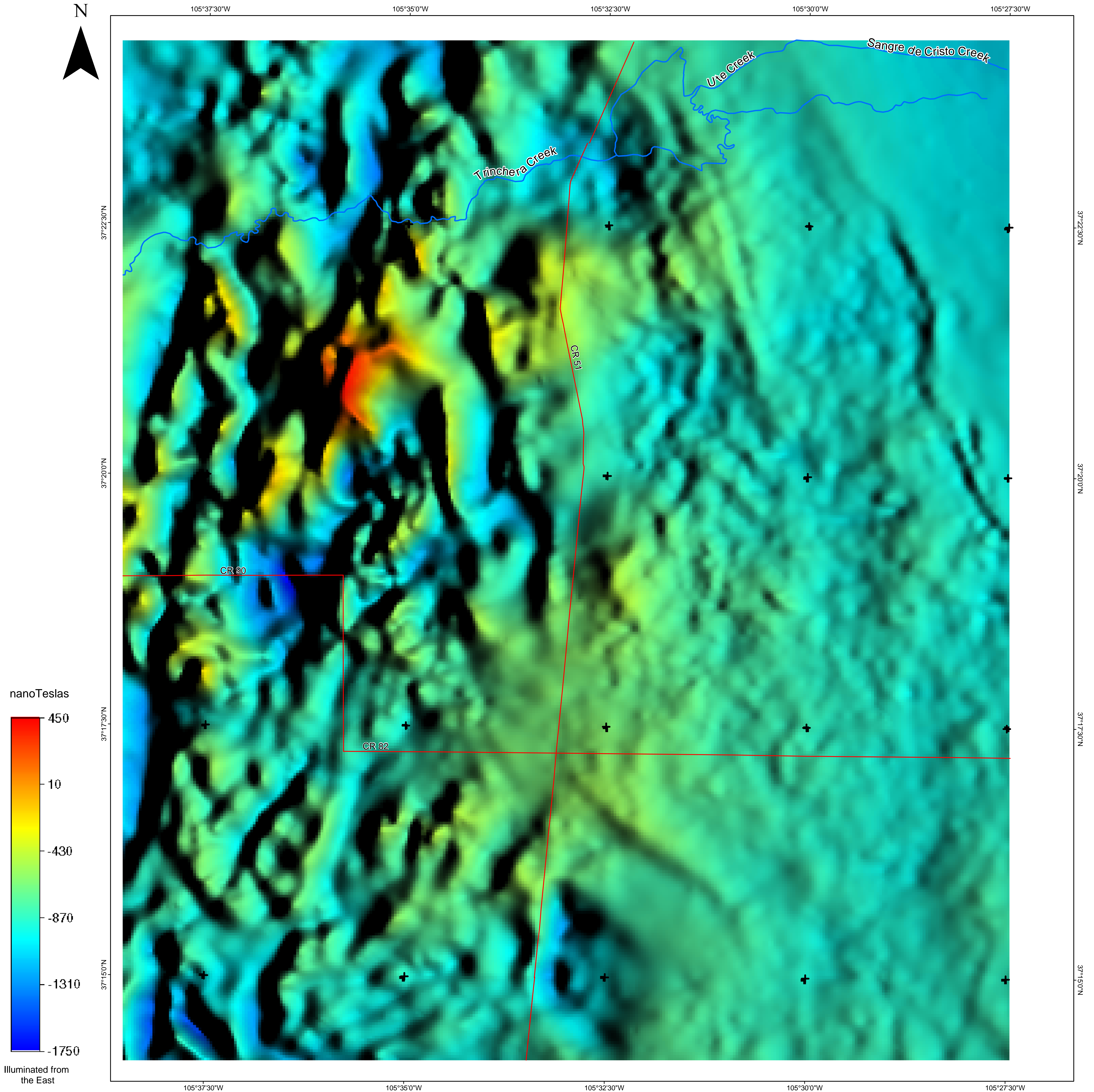
Central San Luis Basin Aeromagnetic Survey Color shaded-relief image of continued, reduced-to-pole (RTP) magnetic data, Blanca Southeast area.
