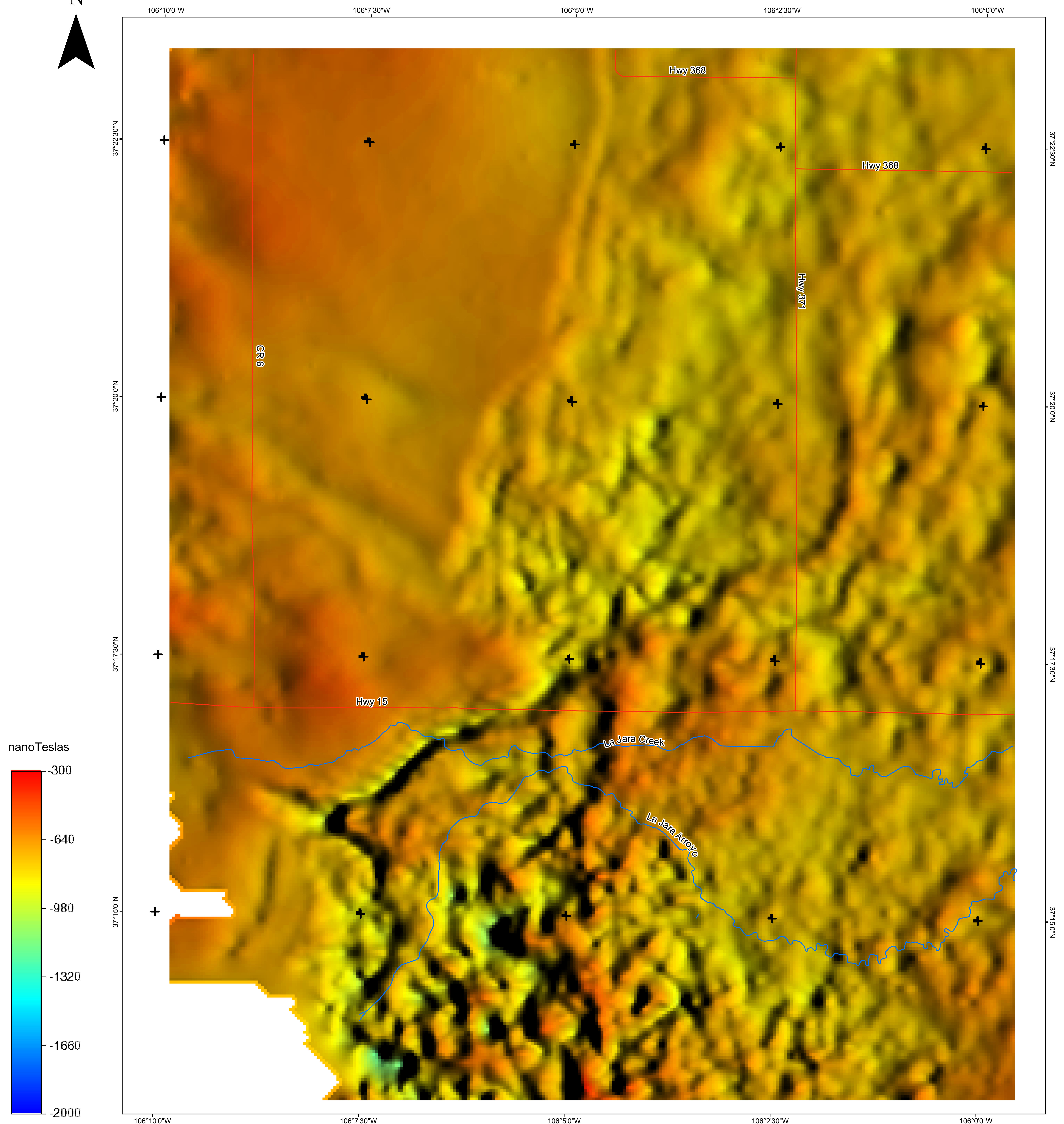
Central San Luis Basin Aeromagnetic Survey Color shaded-relief image of continued, reduced-to-pole (RTP) magnetic data, Capulin area.
