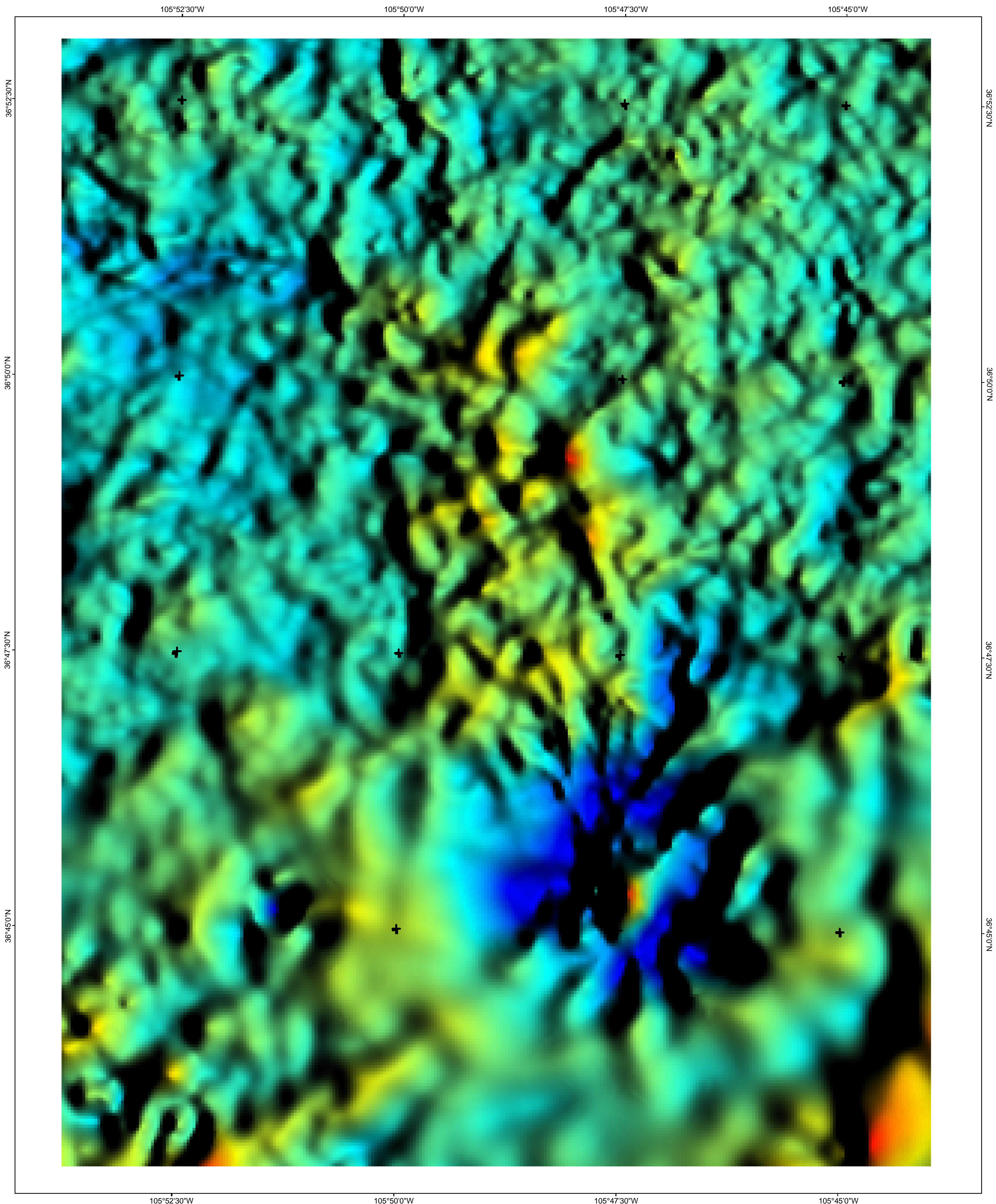
Central San Luis Basin Aeromagnetic Survey Color shaded-relief image of continued, reduced-to-pole (RTP) magnetic data, Cerro de La Olla area.
