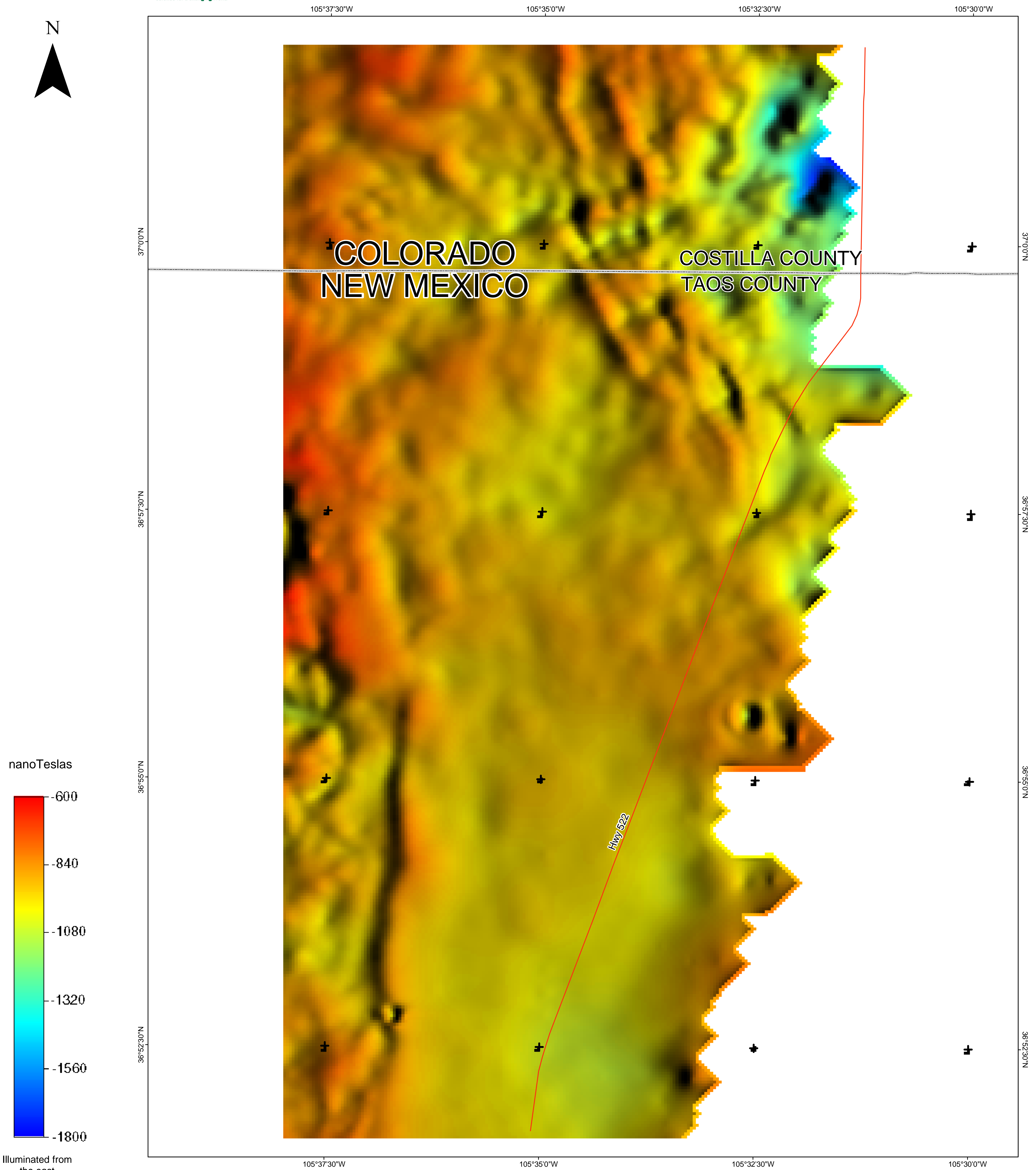
Central San Luis Basin Aeromagnetic Survey Color shaded-relief image of continued, reduced-to-pole (RTP) magnetic data, Costilla area.
