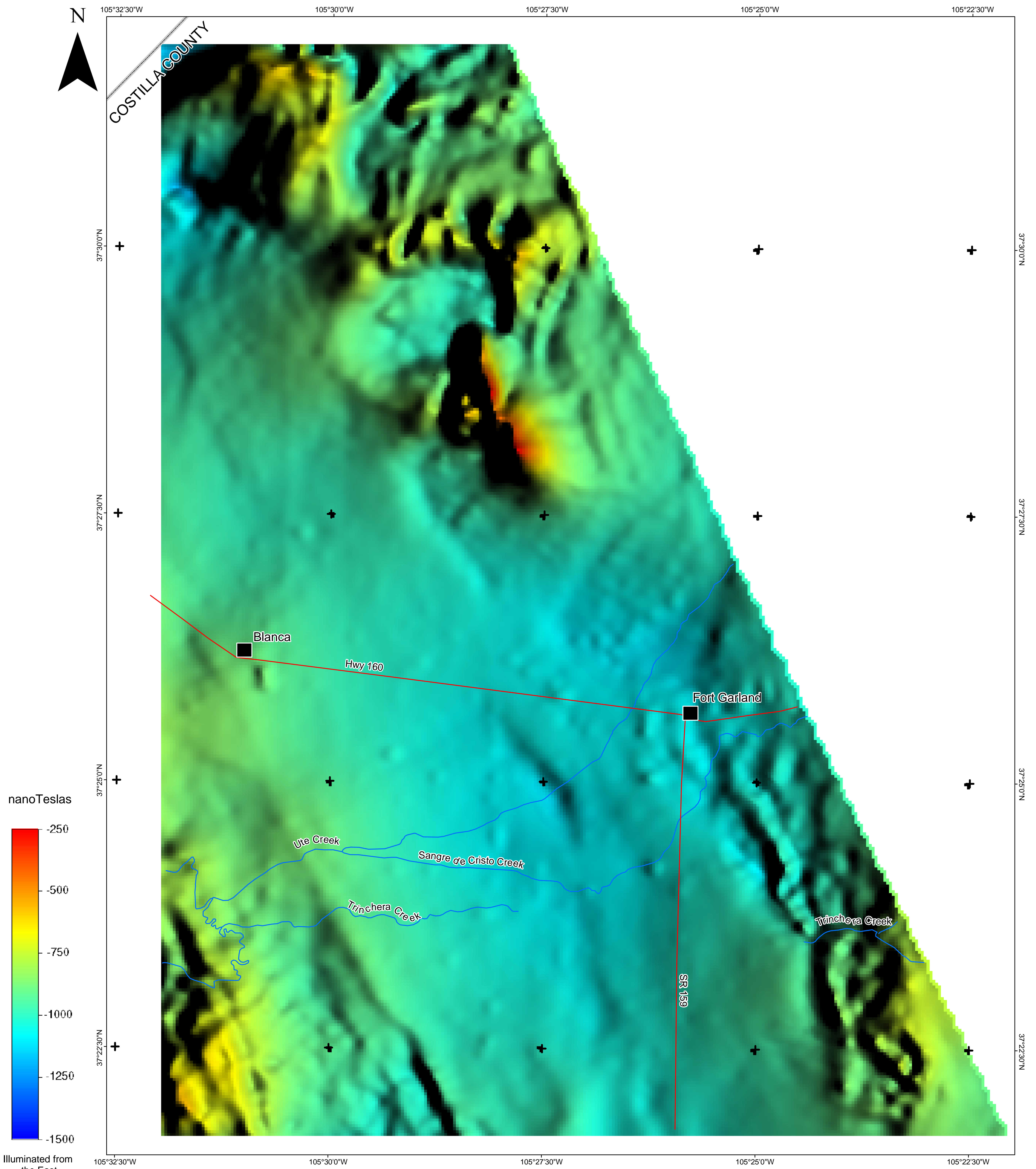
Central San Luis Basin Aeromagnetic Survey Color shaded-relief image of continued, reduced-to-pole (RTP) magnetic data, Fort Garland area.
