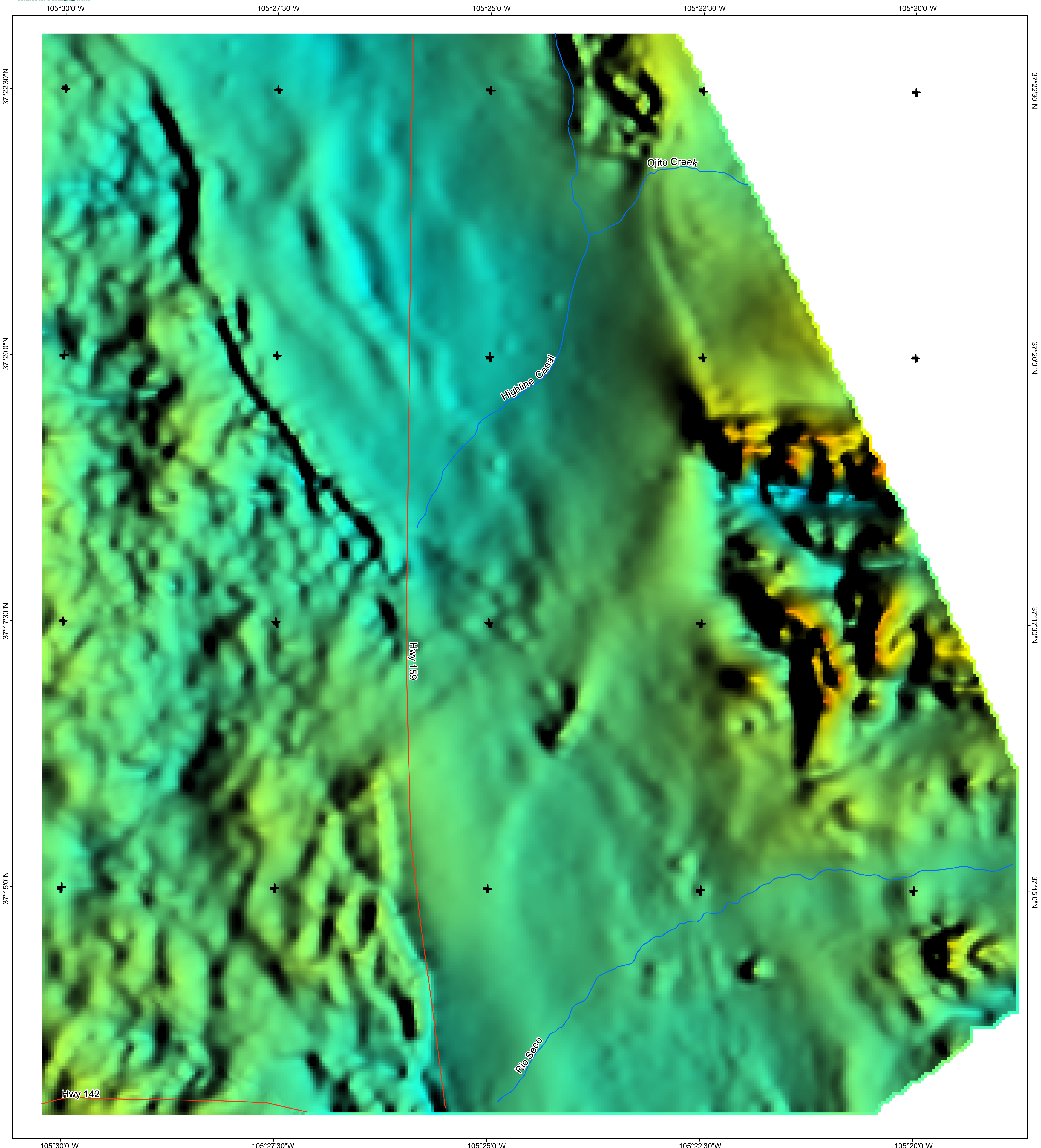
Central San Luis Basin Aeromagnetic Survey Color shaded-relief image of continued, reduced-to-pole(RTP) magnetic data, Fort Garland SW area.
