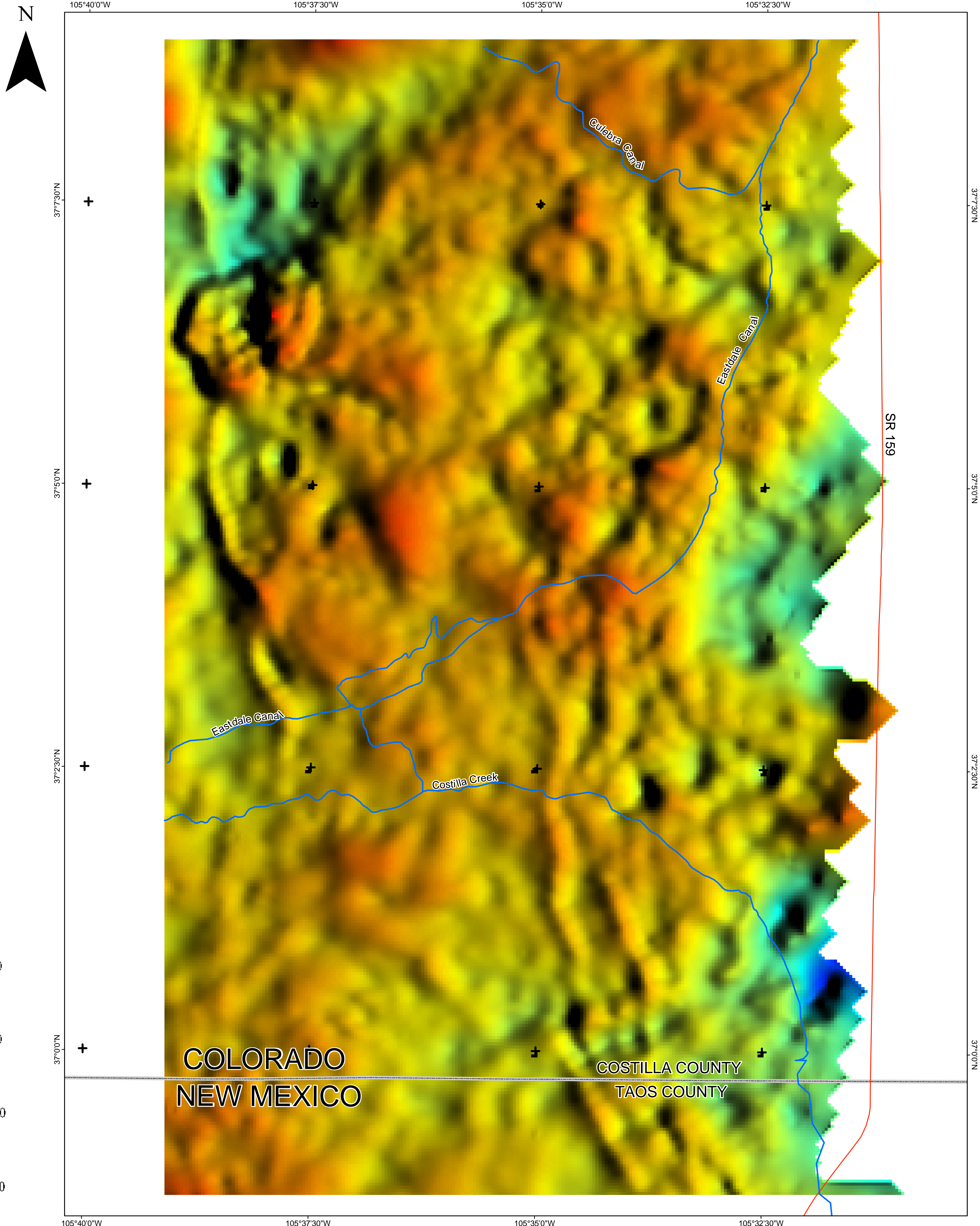
Central San Luis Basin Aeromagnetic Survey Color shaded-relief image of continued, reduced-to-pole (RTP) magnetic data, Garcia area.
