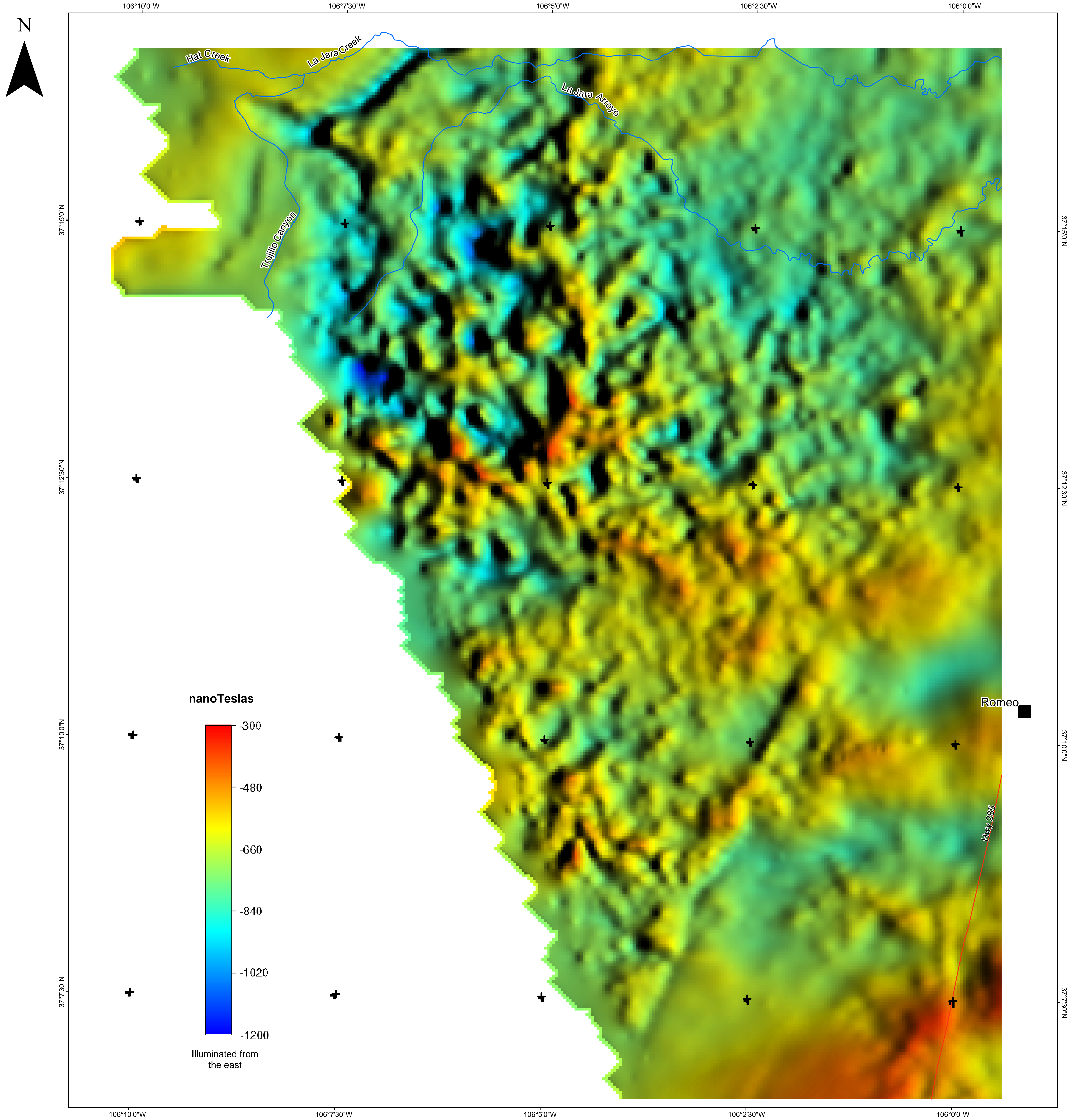
Central San Luis Basin Aeromagnetic Survey Color shaded-relief image of continued, reduced-to-pole (RTP) magnetic data, Goshawk Dam area.
