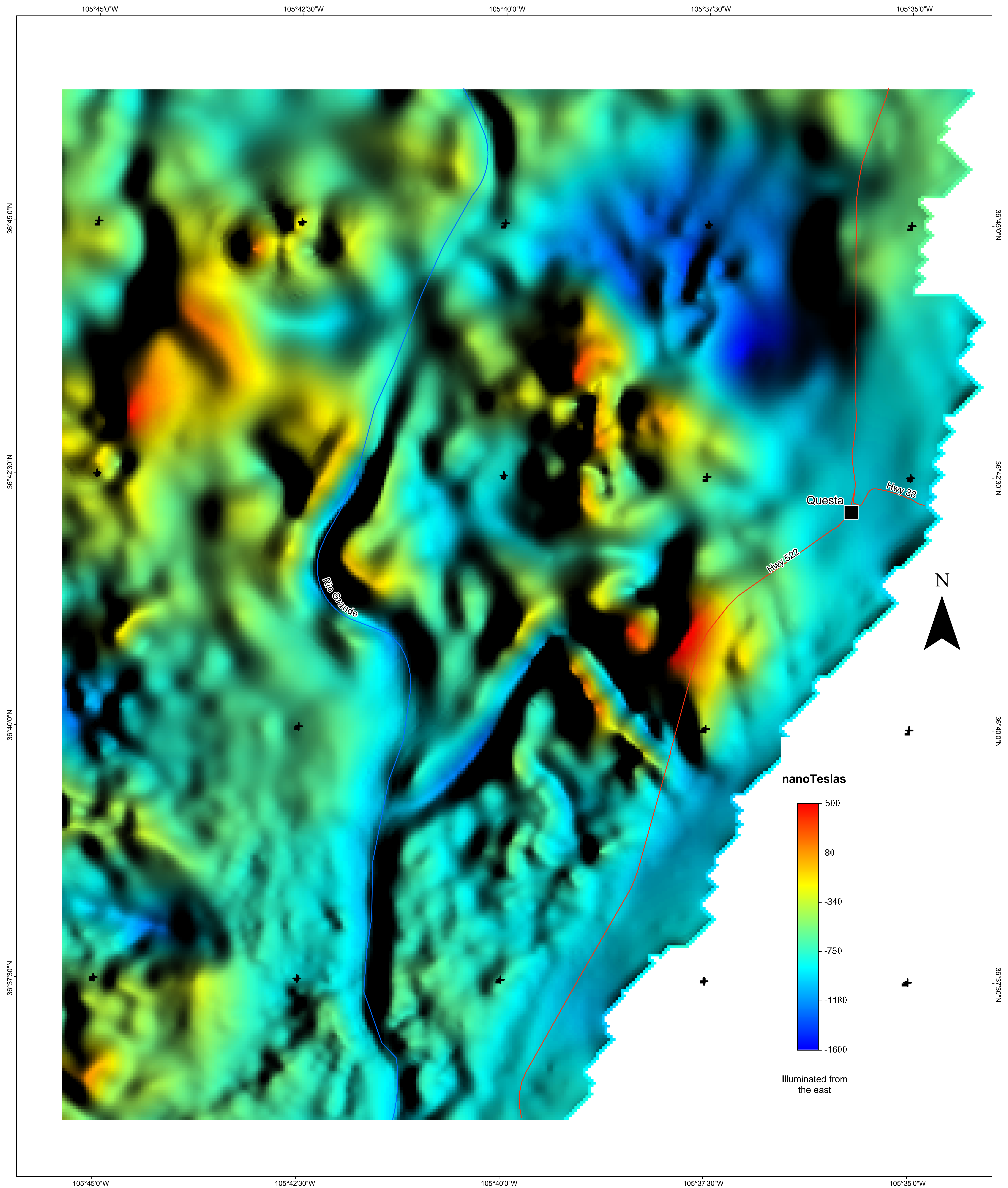
Central San Luis Basin Aeromagnetic Survey Color shaded-relief image of continued, reduced-to-pole (RTP) magnetic data, Guadalupe Mountain area.
